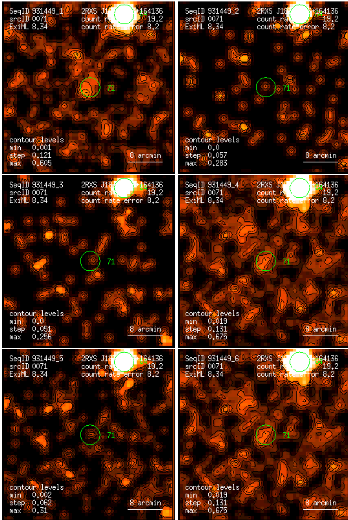
Figure 71: RASS 931449: detection 0071: band rate images, Gaussian filter: (1) PSPC channels 11 – 41, (2) 52 – 90, (3) 91 – 201, (4) 11 – 235, (5) 52 – 201, (6) 11 – 201. Broad band rates in counts/ks. Band rate contour levels in counts/ks/arcmin 2 .
