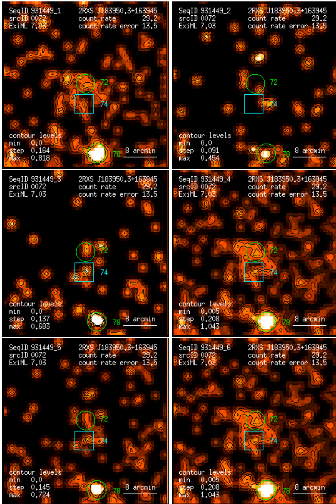
Figure 72: RASS 931449: detection 0072: band rate images, Gaussian filter: (1) PSPC channels 11 – 41, (2) 52 – 90, (3) 91 – 201, (4) 11 – 235, (5) 52 – 201, (6) 11 – 201. Broad band rates in counts/ks. Band rate contour levels in counts/ks/arcmin 2 .
