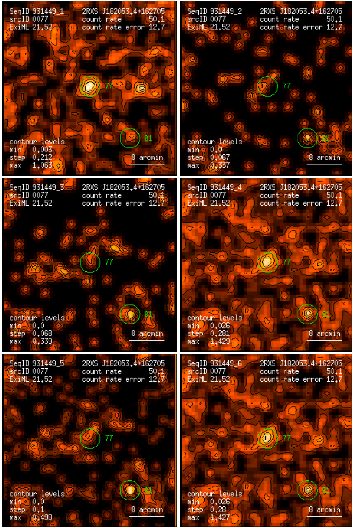
Figure 77: RASS 931449: detection 0077: band rate images, Gaussian filter: (1) PSPC channels 11 – 41, (2) 52 – 90, (3) 91 – 201, (4) 11 – 235, (5) 52 – 201, (6) 11 – 201. Broad band rates in counts/ks. Band rate contour levels in counts/ks/arcmin 2 .
