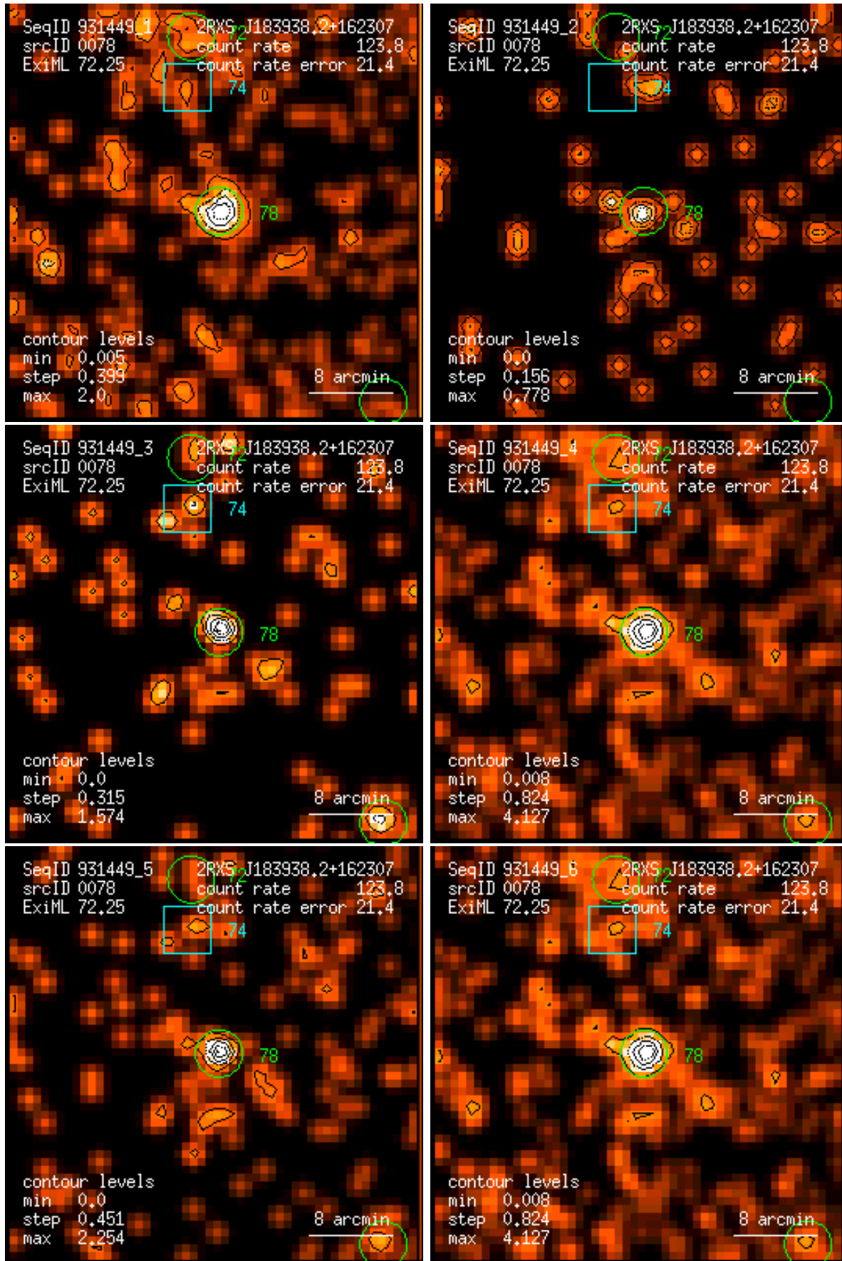
Figure 78: RASS 931449: detection 0078: band rate images, Gaussian filter: (1) PSPC channels 11 – 41, (2) 52 – 90, (3) 91 – 201, (4) 11 – 235, (5) 52 – 201, (6) 11 – 201. Broad band rates in counts/ks. Band rate contour levels in counts/ks/arcmin 2 .
