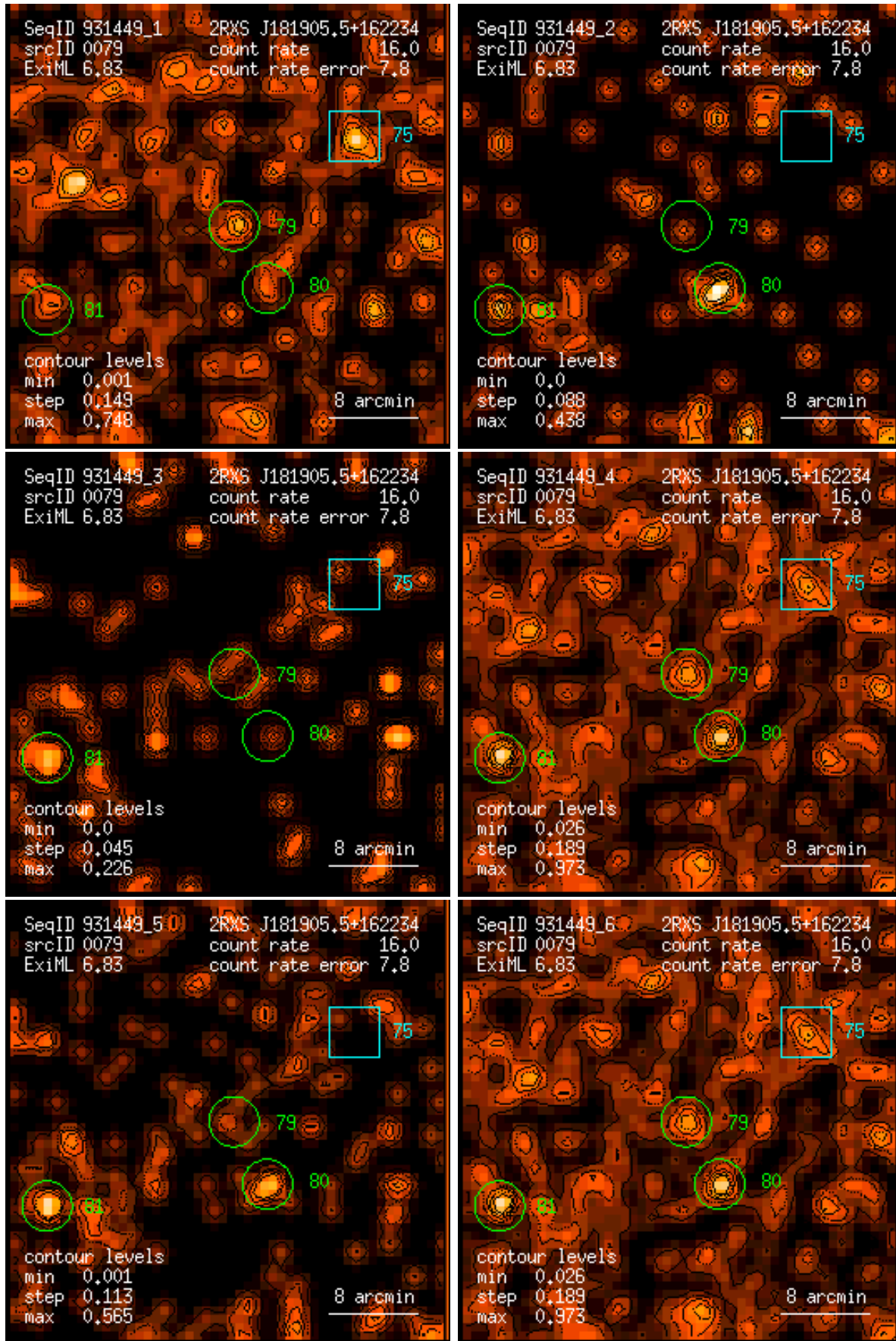
Figure 79: RASS 931449: detection 0079: band rate images, Gaussian filter: (1) PSPC channels 11 – 41, (2) 52 – 90, (3) 91 – 201, (4) 11 – 235, (5) 52 – 201, (6) 11 – 201. Broad band rates in counts/ks. Band rate contour levels in counts/ks/arcmin 2 .
