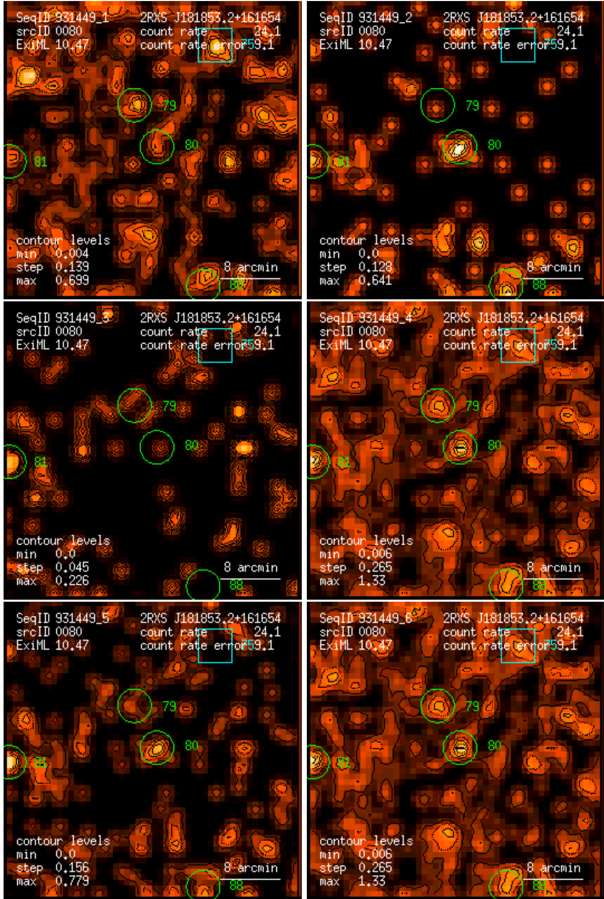
Figure 80: RASS 931449: detection 0080: band rate images, Gaussian filter: (1) PSPC channels 11 – 41, (2) 52 – 90, (3) 91 – 201, (4) 11 – 235, (5) 52 – 201, (6) 11 – 201. Broad band rates in counts/ks. Band rate contour levels in counts/ks/arcmin 2 .
