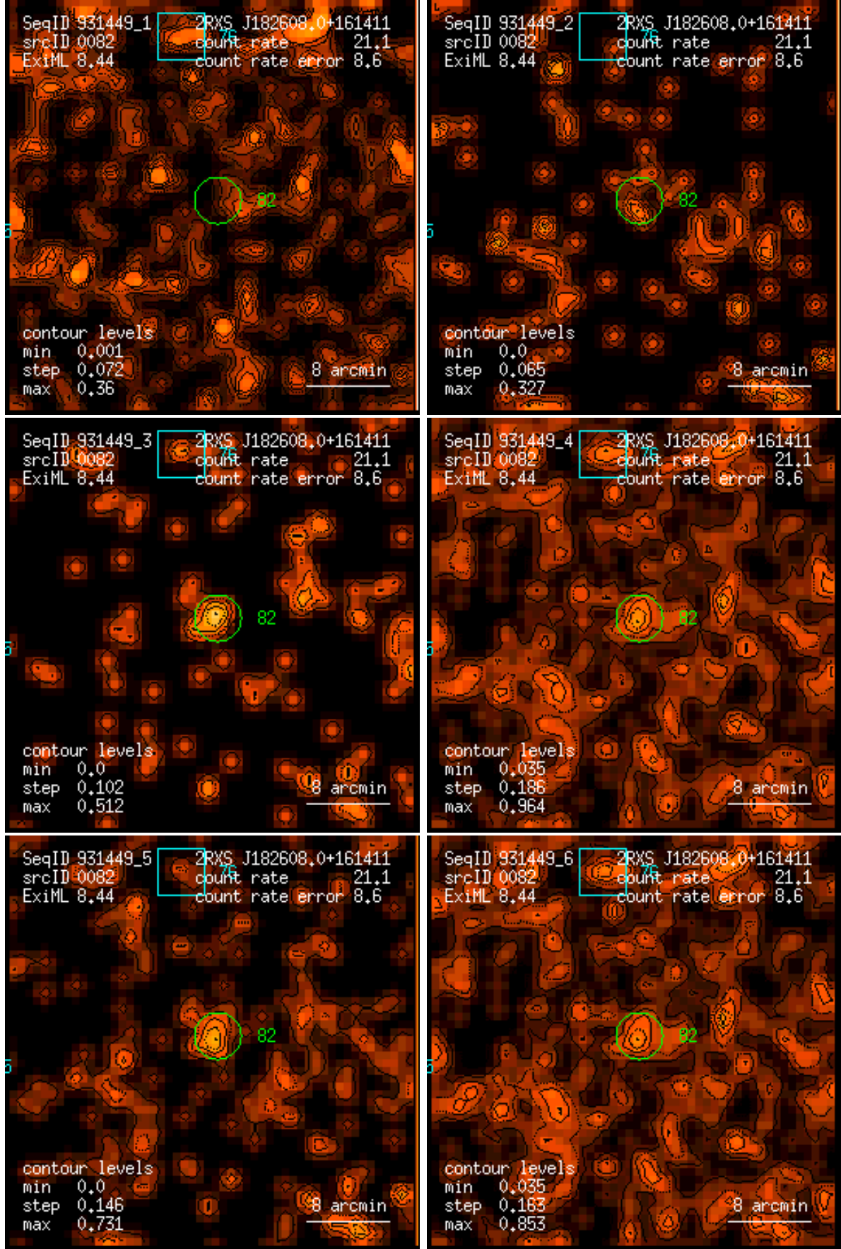
Figure 82: RASS 931449: detection 0082: band rate images, Gaussian filter: (1) PSPC channels 11 – 41, (2) 52 – 90, (3) 91 – 201, (4) 11 – 235, (5) 52 – 201, (6) 11 – 201. Broad band rates in counts/ks. Band rate contour levels in counts/ks/arcmin 2 .
