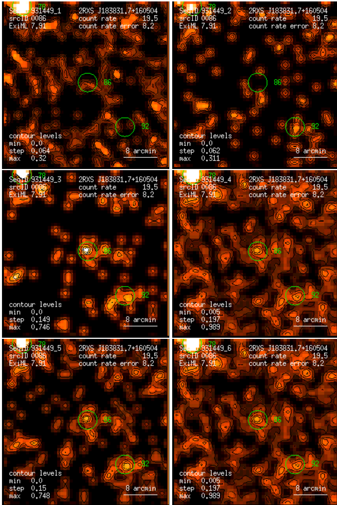
Figure 86: RASS 931449: detection 0086: band rate images, Gaussian filter: (1) PSPC channels 11 – 41, (2) 52 – 90, (3) 91 – 201, (4) 11 – 235, (5) 52 – 201, (6) 11 – 201. Broad band rates in counts/ks. Band rate contour levels in counts/ks/arcmin 2 .
