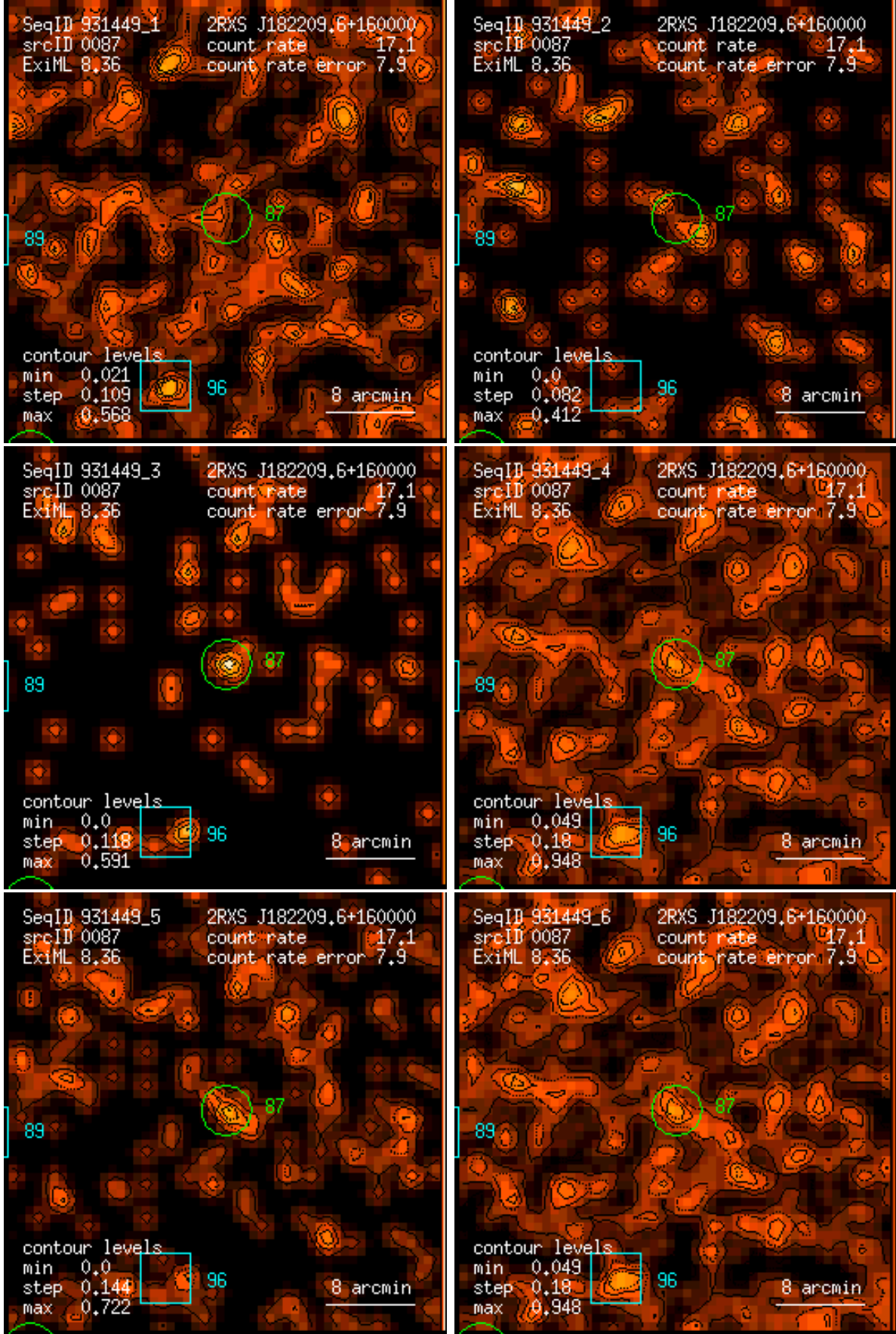
Figure 87: RASS 931449: detection 0087: band rate images, Gaussian filter: (1) PSPC channels 11 – 41, (2) 52 – 90, (3) 91 – 201, (4) 11 – 235, (5) 52 – 201, (6) 11 – 201. Broad band rates in counts/ks. Band rate contour levels in counts/ks/arcmin 2 .
