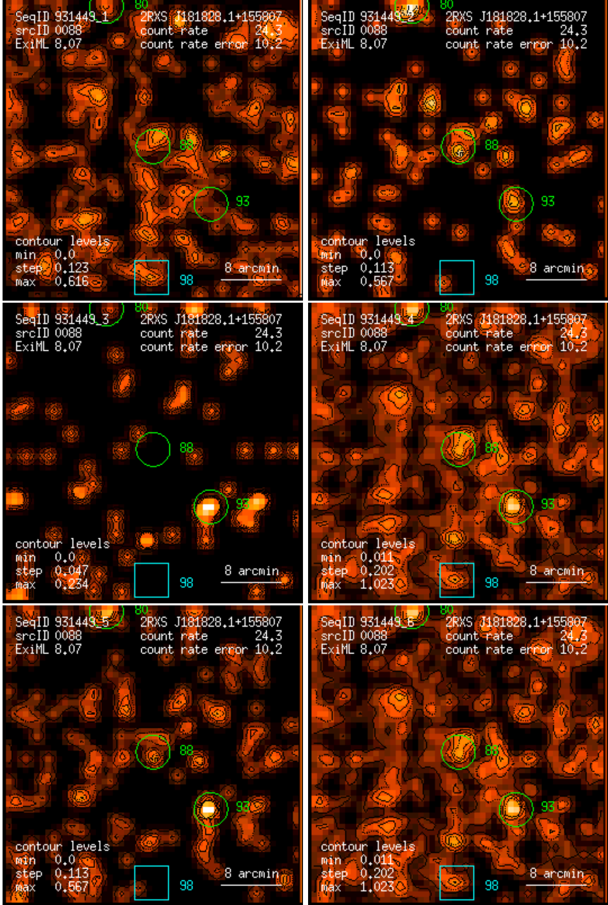
Figure 88: RASS 931449: detection 0088: band rate images, Gaussian filter: (1) PSPC channels 11 – 41, (2) 52 – 90, (3) 91 – 201, (4) 11 – 235, (5) 52 – 201, (6) 11 – 201. Broad band rates in counts/ks. Band rate contour levels in counts/ks/arcmin 2 .
