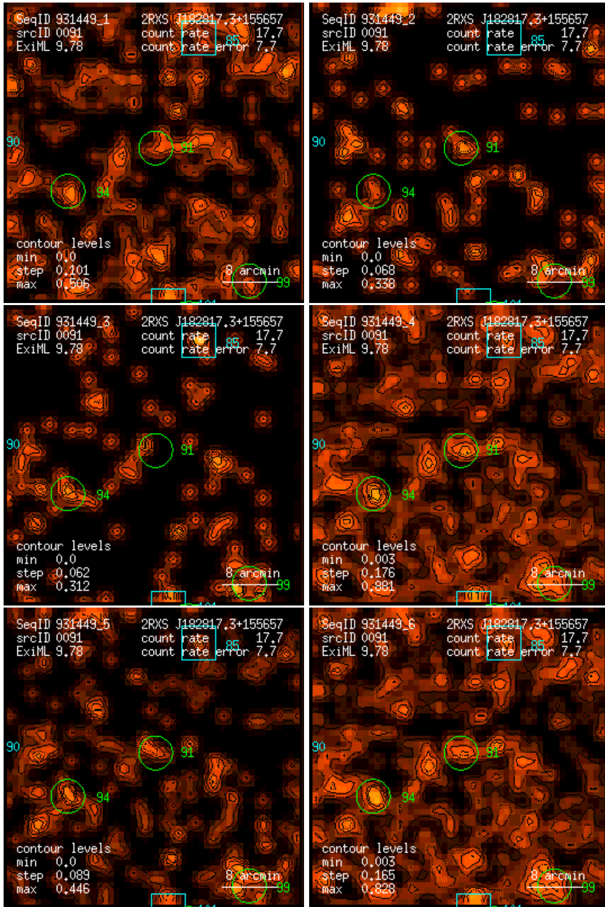
Figure 91: RASS 931449: detection 0091: band rate images, Gaussian filter: (1) PSPC channels 11 – 41, (2) 52 – 90, (3) 91 – 201, (4) 11 – 235, (5) 52 – 201, (6) 11 – 201. Broad band rates in counts/ks. Band rate contour levels in counts/ks/arcmin 2 .
