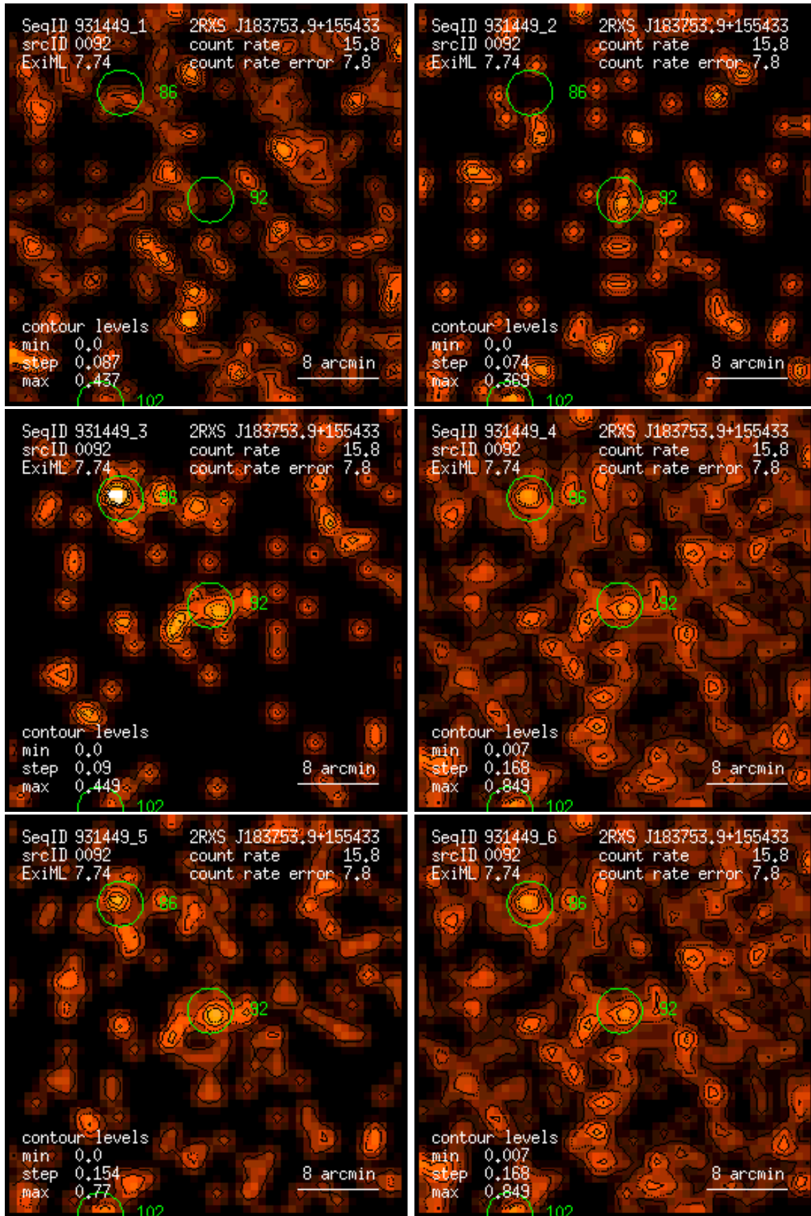
Figure 92: RASS 931449: detection 0092: band rate images, Gaussian filter: (1) PSPC channels 11 – 41, (2) 52 – 90, (3) 91 – 201, (4) 11 – 235, (5) 52 – 201, (6) 11 – 201. Broad band rates in counts/ks. Band rate contour levels in counts/ks/arcmin 2 .
