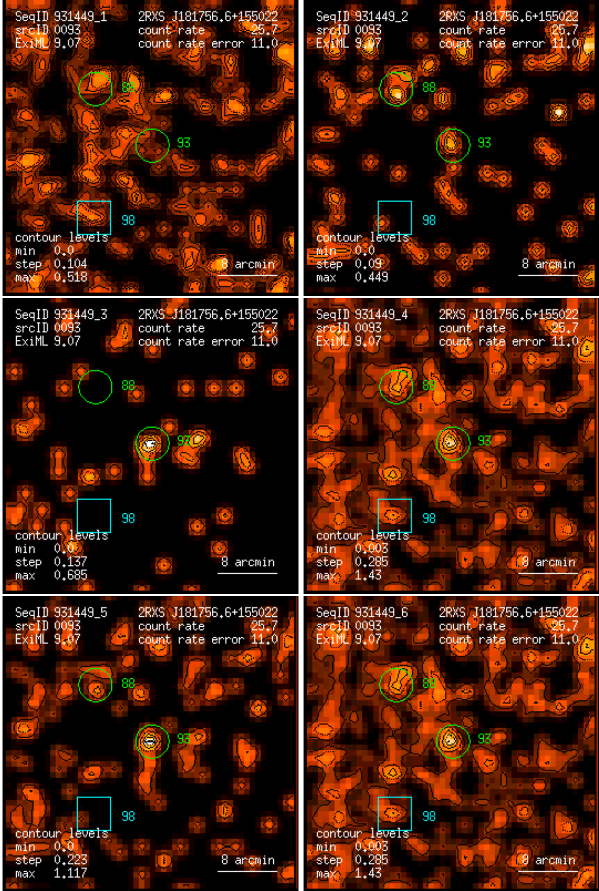
Figure 93: RASS 931449: detection 0093: band rate images, Gaussian filter: (1) PSPC channels 11 – 41, (2) 52 – 90, (3) 91 – 201, (4) 11 – 235, (5) 52 – 201, (6) 11 – 201. Broad band rates in counts/ks. Band rate contour levels in counts/ks/arcmin 2 .
