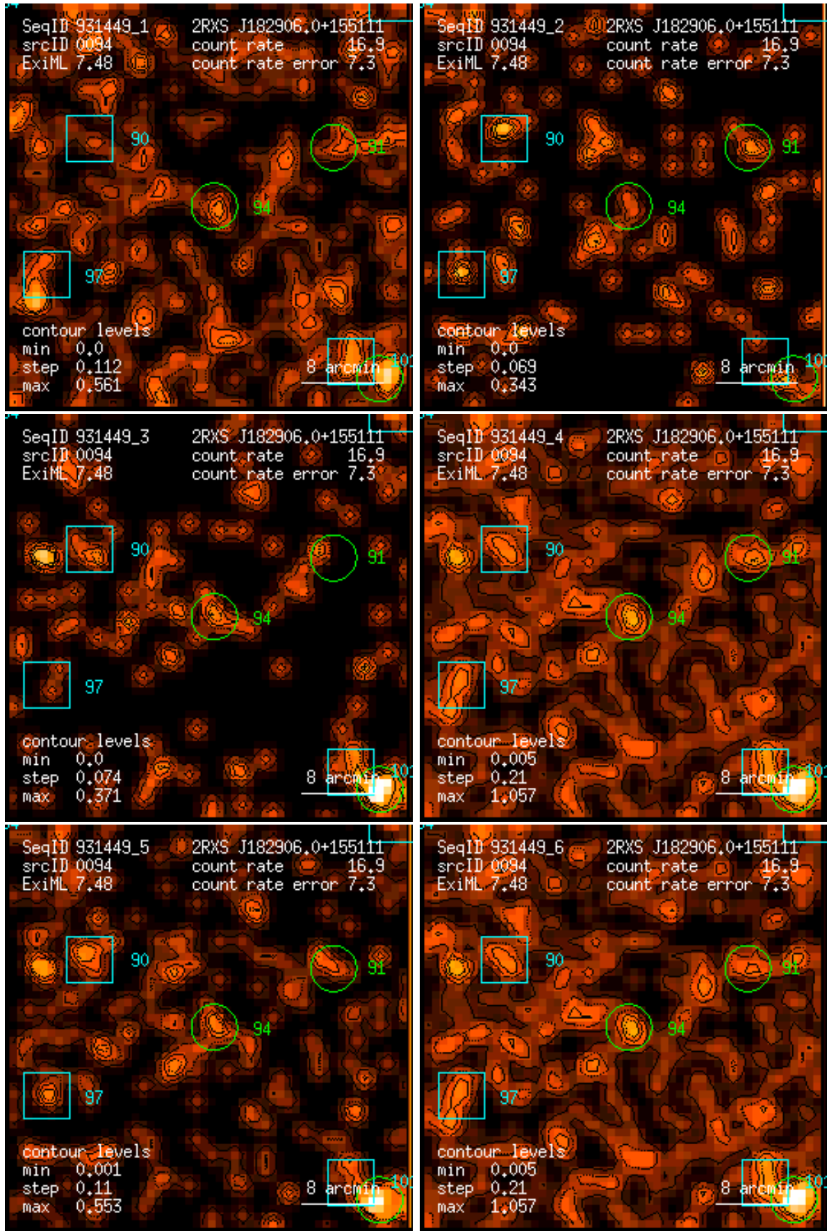
Figure 94: RASS 931449: detection 0094: band rate images, Gaussian filter: (1) PSPC channels 11 – 41, (2) 52 – 90, (3) 91 – 201, (4) 11 – 235, (5) 52 – 201, (6) 11 – 201. Broad band rates in counts/ks. Band rate contour levels in counts/ks/arcmin 2 .
