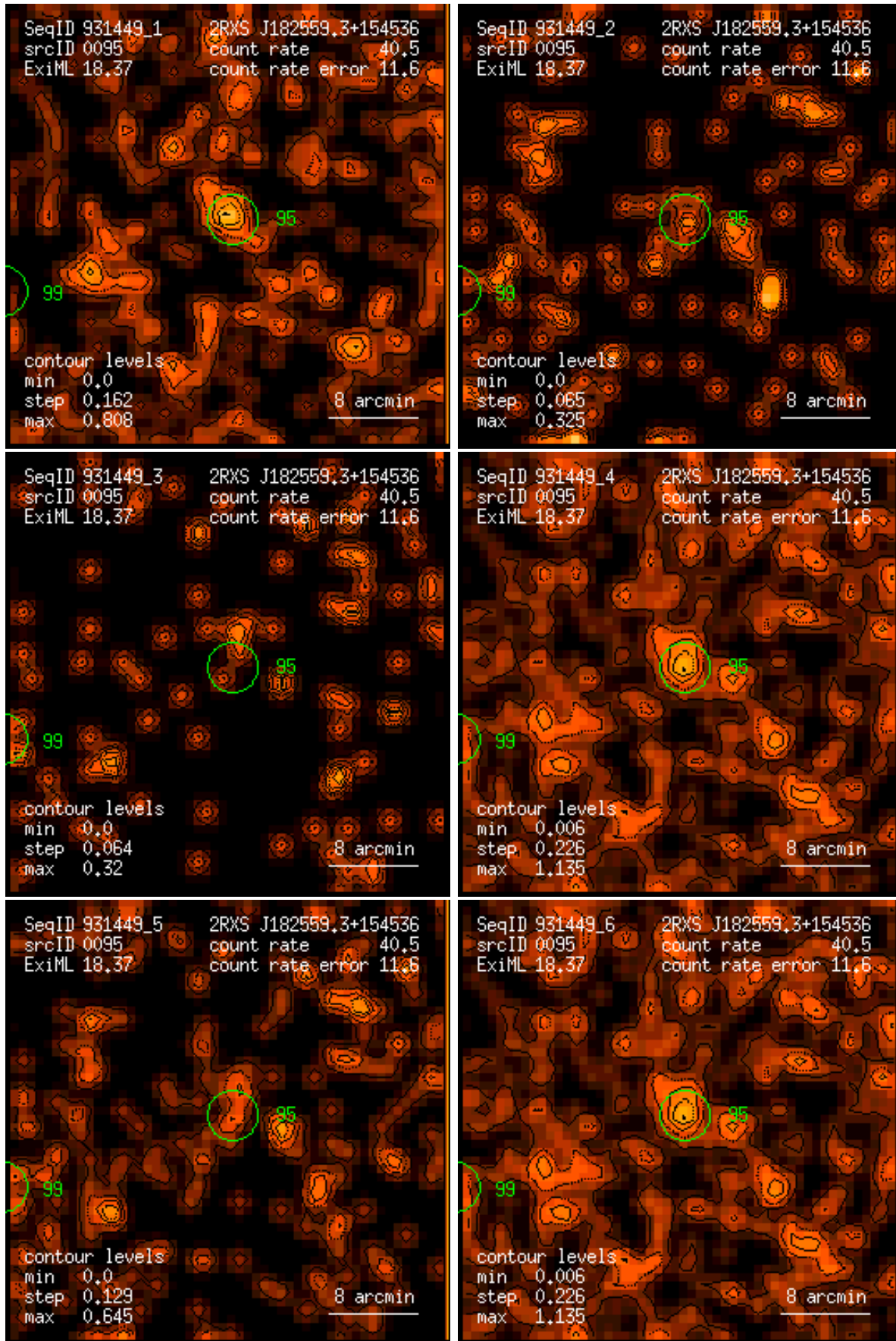
Figure 95: RASS 931449: detection 0095: band rate images, Gaussian filter: (1) PSPC channels 11 – 41, (2) 52 – 90, (3) 91 – 201, (4) 11 – 235, (5) 52 – 201, (6) 11 – 201. Broad band rates in counts/ks. Band rate contour levels in counts/ks/arcmin 2 .
