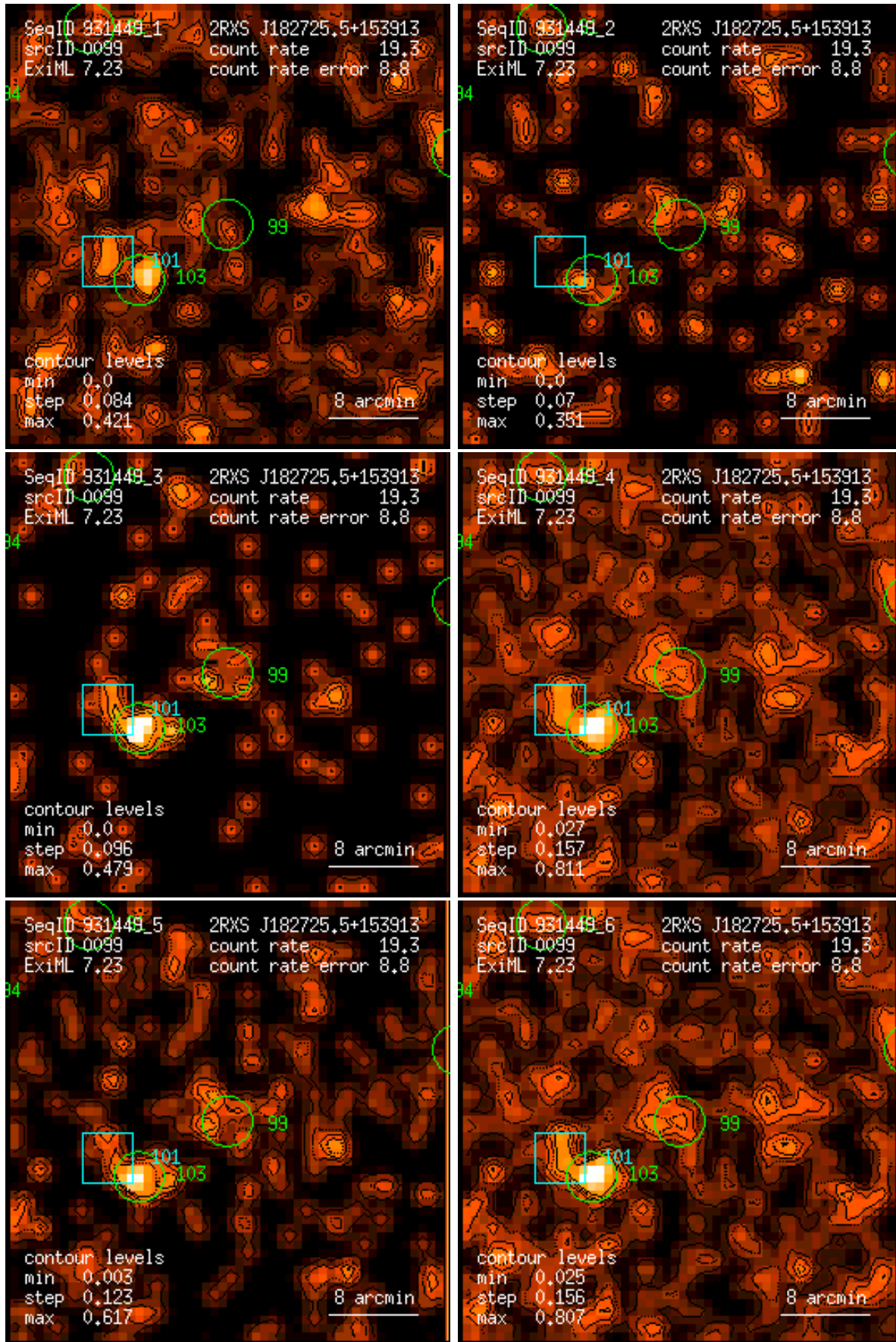
Figure 99: RASS 931449: detection 0099: band rate images, Gaussian filter: (1) PSPC channels 11 – 41, (2) 52 – 90, (3) 91 – 201, (4) 11 – 235, (5) 52 – 201, (6) 11 – 201. Broad band rates in counts/ks. Band rate contour levels in counts/ks/arcmin 2 .
