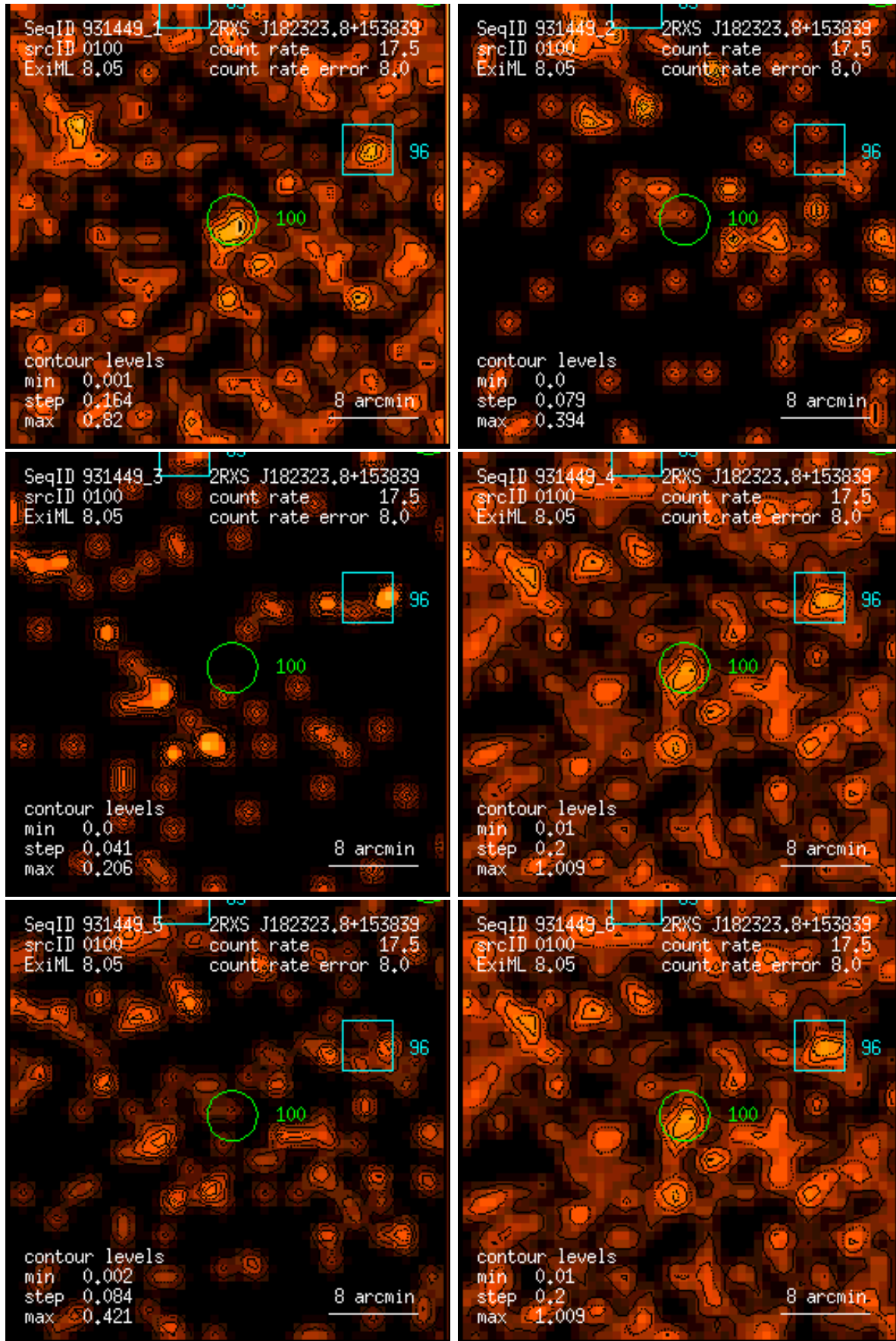
Figure 100: RASS 931449: detection 0100: band rate images, Gaussian filter: (1) PSPC channels 11 – 41, (2) 52 – 90, (3) 91 – 201, (4) 11 – 235, (5) 52 – 201, (6) 11 – 201. Broad band rates in counts/ks. Band rate contour levels in counts/ks/arcmin 2 .
