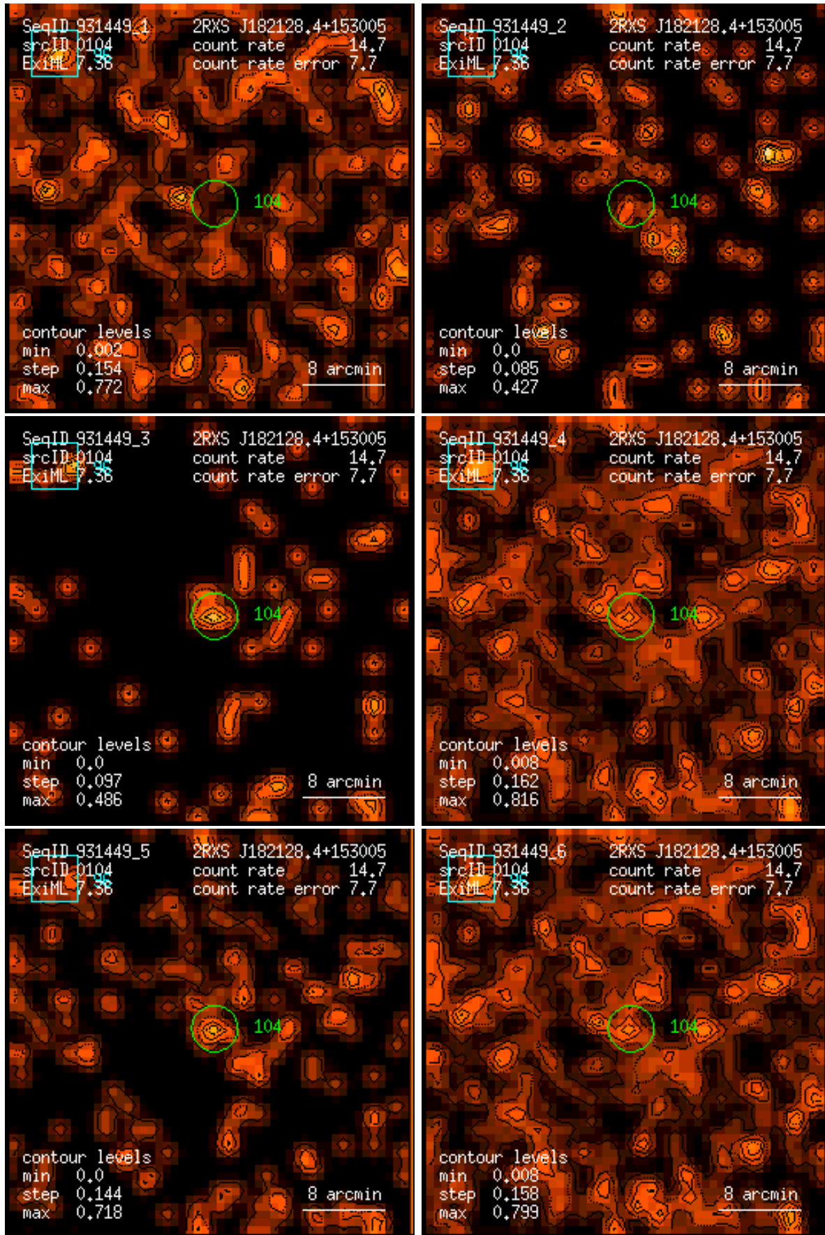
Figure 104: RASS 931449: detection 0104: band rate images, Gaussian filter: (1) PSPC channels 11 – 41, (2) 52 – 90, (3) 91 – 201, (4) 11 – 235, (5) 52 – 201, (6) 11 – 201. Broad band rates in counts/ks. Band rate contour levels in counts/ks/arcmin 2 .
