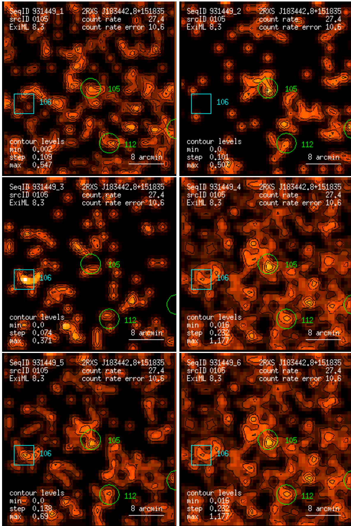
Figure 105: RASS 931449: detection 0105: band rate images, Gaussian filter: (1) PSPC channels 11 – 41, (2) 52 – 90, (3) 91 – 201, (4) 11 – 235, (5) 52 – 201, (6) 11 – 201. Broad band rates in counts/ks. Band rate contour levels in counts/ks/arcmin 2 .
