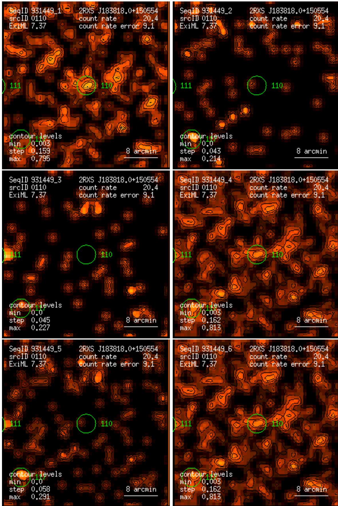
Figure 110: RASS 931449: detection 0110: band rate images, Gaussian filter: (1) PSPC channels 11 – 41, (2) 52 – 90, (3) 91 – 201, (4) 11 – 235, (5) 52 – 201, (6) 11 – 201. Broad band rates in counts/ks. Band rate contour levels in counts/ks/arcmin 2 .
