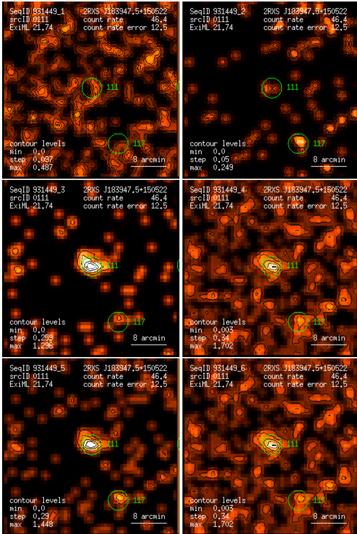
Figure 111: RASS 931449: detection 0111: band rate images, Gaussian filter: (1) PSPC channels 11 – 41, (2) 52 – 90, (3) 91 – 201, (4) 11 – 235, (5) 52 – 201, (6) 11 – 201. Broad band rates in counts/ks. Band rate contour levels in counts/ks/arcmin 2 .
