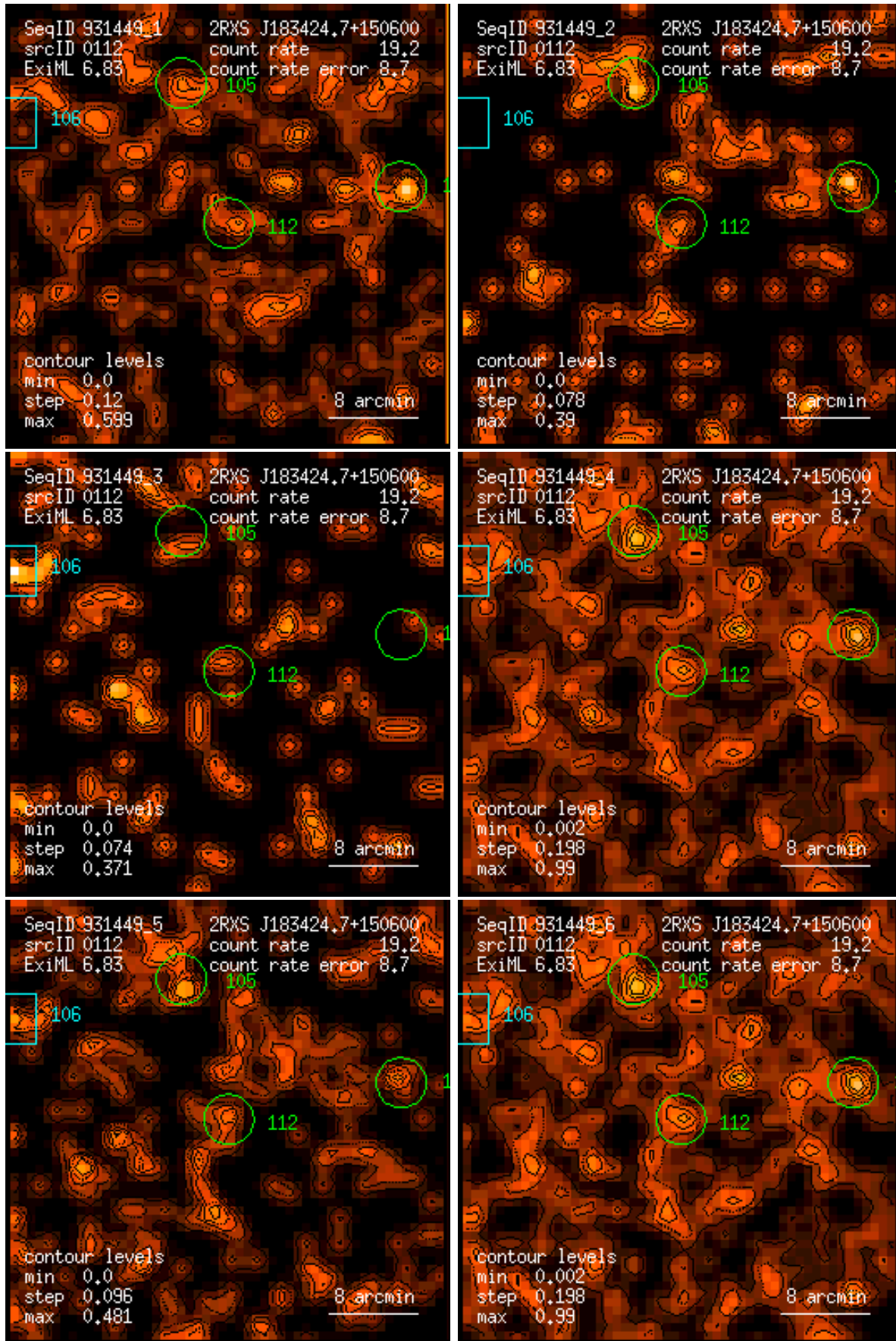
Figure 112: RASS 931449: detection 0112: band rate images, Gaussian filter: (1) PSPC channels 11 – 41, (2) 52 – 90, (3) 91 – 201, (4) 11 – 235, (5) 52 – 201, (6) 11 – 201. Broad band rates in counts/ks. Band rate contour levels in counts/ks/arcmin 2 .
