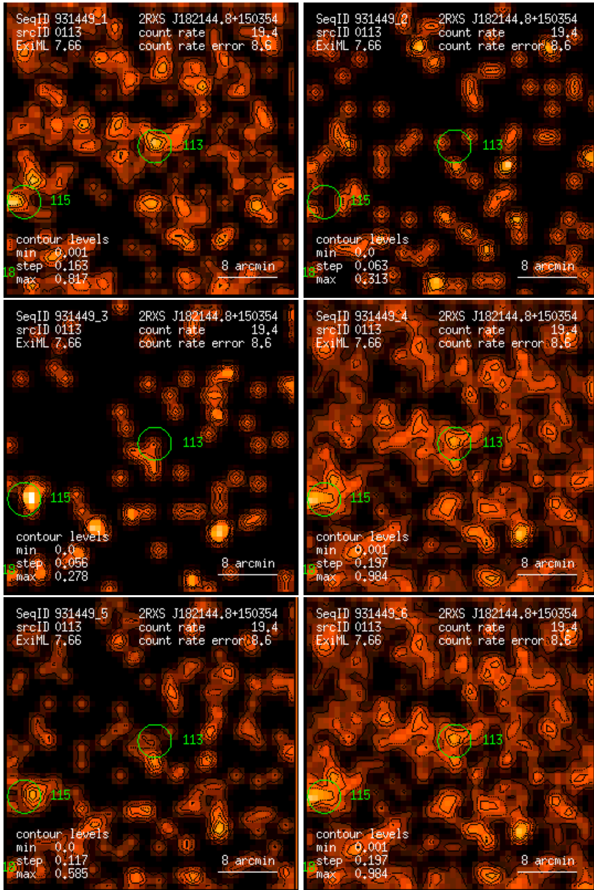
Figure 113: RASS 931449: detection 0113: band rate images, Gaussian filter: (1) PSPC channels 11 – 41, (2) 52 – 90, (3) 91 – 201, (4) 11 – 235, (5) 52 – 201, (6) 11 – 201. Broad band rates in counts/ks. Band rate contour levels in counts/ks/arcmin 2 .
