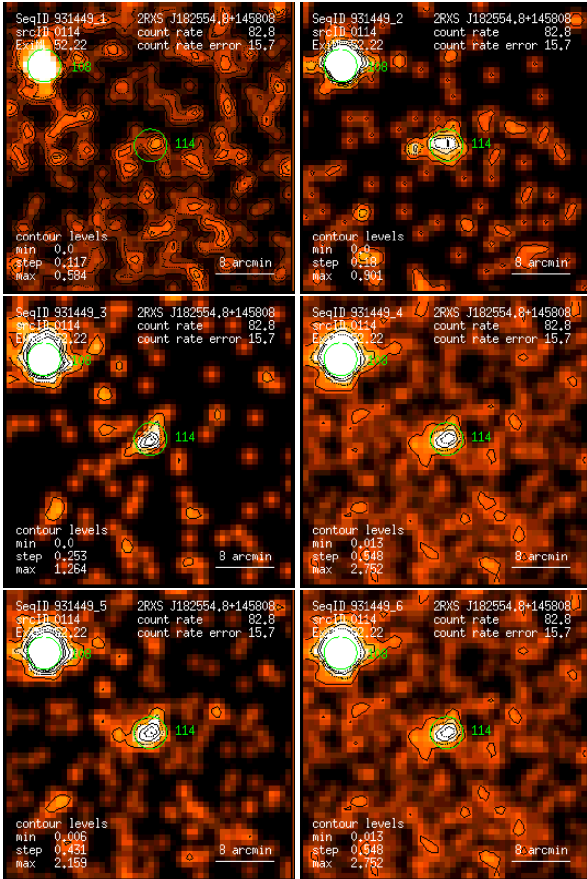
Figure 114: RASS 931449: detection 0114: band rate images, Gaussian filter: (1) PSPC channels 11 – 41, (2) 52 – 90, (3) 91 – 201, (4) 11 – 235, (5) 52 – 201, (6) 11 – 201. Broad band rates in counts/ks. Band rate contour levels in counts/ks/arcmin 2 .
