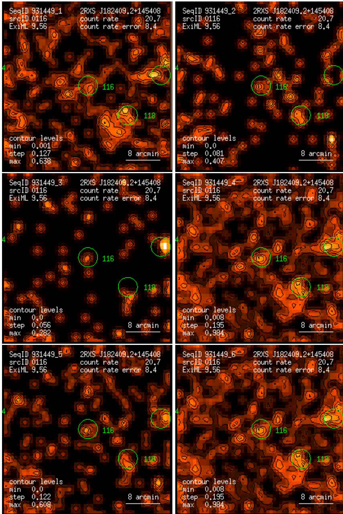
Figure 116: RASS 931449: detection 0116: band rate images, Gaussian filter: (1) PSPC channels 11 – 41, (2) 52 – 90, (3) 91 – 201, (4) 11 – 235, (5) 52 – 201, (6) 11 – 201. Broad band rates in counts/ks. Band rate contour levels in counts/ks/arcmin 2 .
