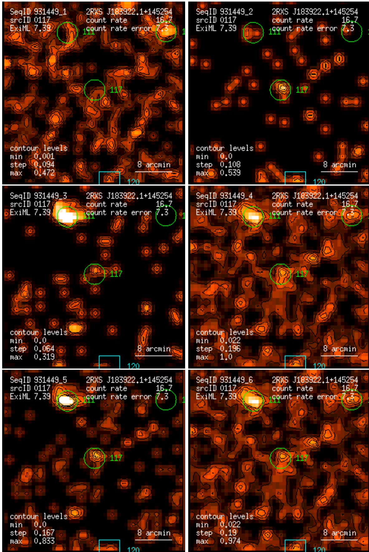
Figure 117: RASS 931449: detection 0117: band rate images, Gaussian filter: (1) PSPC channels 11 – 41, (2) 52 – 90, (3) 91 – 201, (4) 11 – 235, (5) 52 – 201, (6) 11 – 201. Broad band rates in counts/ks. Band rate contour levels in counts/ks/arcmin 2 .
