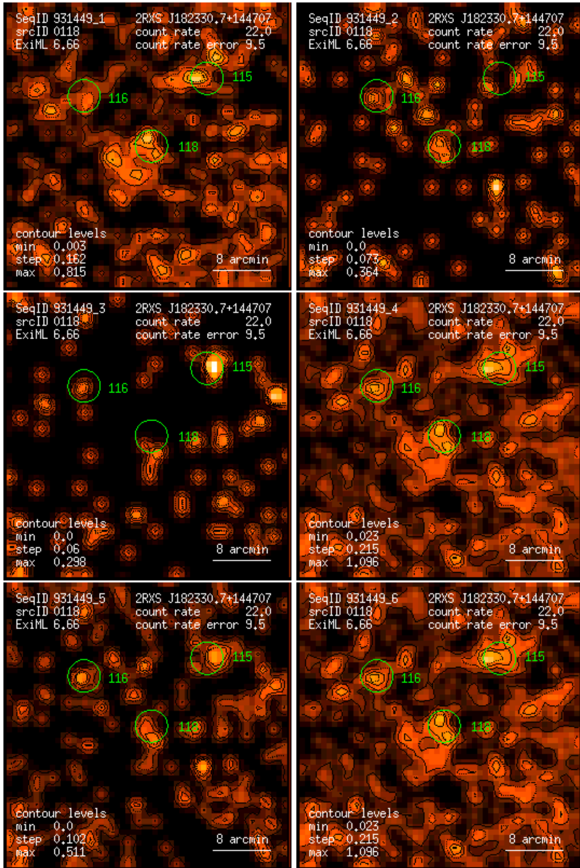
Figure 118: RASS 931449: detection 0118: band rate images, Gaussian filter: (1) PSPC channels 11 – 41, (2) 52 – 90, (3) 91 – 201, (4) 11 – 235, (5) 52 – 201, (6) 11 – 201. Broad band rates in counts/ks. Band rate contour levels in counts/ks/arcmin 2 .
