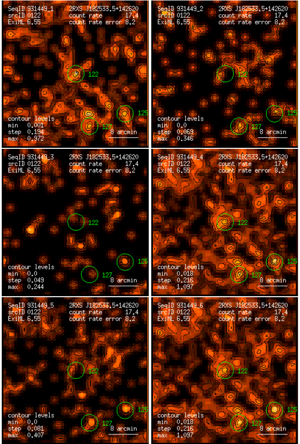
Figure 122: RASS 931449: detection 0122: band rate images, Gaussian filter: (1) PSPC channels 11 – 41, (2) 52 – 90, (3) 91 – 201, (4) 11 – 235, (5) 52 – 201, (6) 11 – 201. Broad band rates in counts/ks. Band rate contour levels in counts/ks/arcmin 2 .
