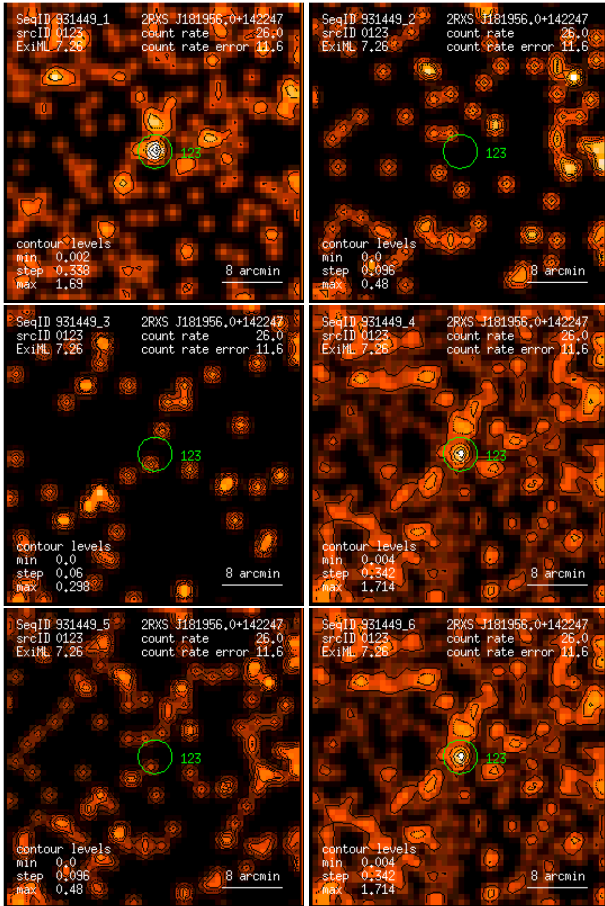
Figure 123: RASS 931449: detection 0123: band rate images, Gaussian filter: (1) PSPC channels 11 – 41, (2) 52 – 90, (3) 91 – 201, (4) 11 – 235, (5) 52 – 201, (6) 11 – 201. Broad band rates in counts/ks. Band rate contour levels in counts/ks/arcmin 2 .
