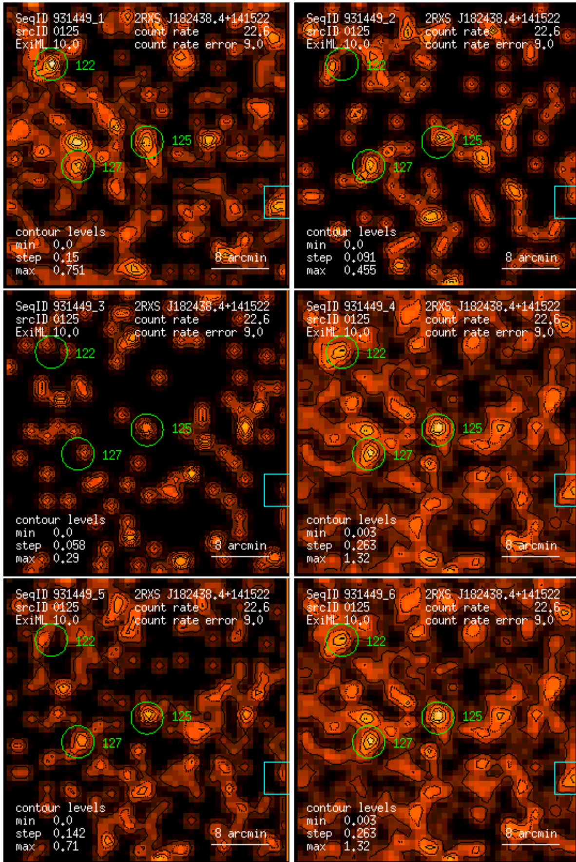
Figure 125: RASS 931449: detection 0125: band rate images, Gaussian filter: (1) PSPC channels 11 – 41, (2) 52 – 90, (3) 91 – 201, (4) 11 – 235, (5) 52 – 201, (6) 11 – 201. Broad band rates in counts/ks. Band rate contour levels in counts/ks/arcmin 2 .
