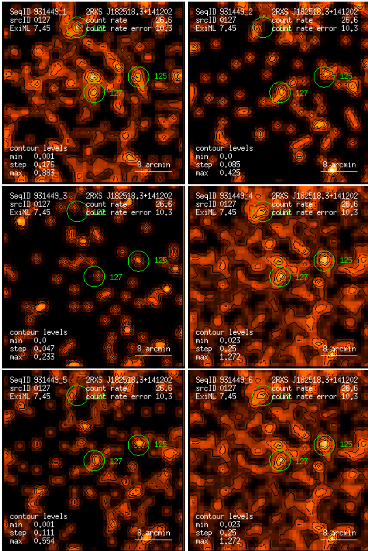
Figure 127: RASS 931449: detection 0127: band rate images, Gaussian filter: (1) PSPC channels 11 – 41, (2) 52 – 90, (3) 91 – 201, (4) 11 – 235, (5) 52 – 201, (6) 11 – 201. Broad band rates in counts/ks. Band rate contour levels in counts/ks/arcmin 2 .
