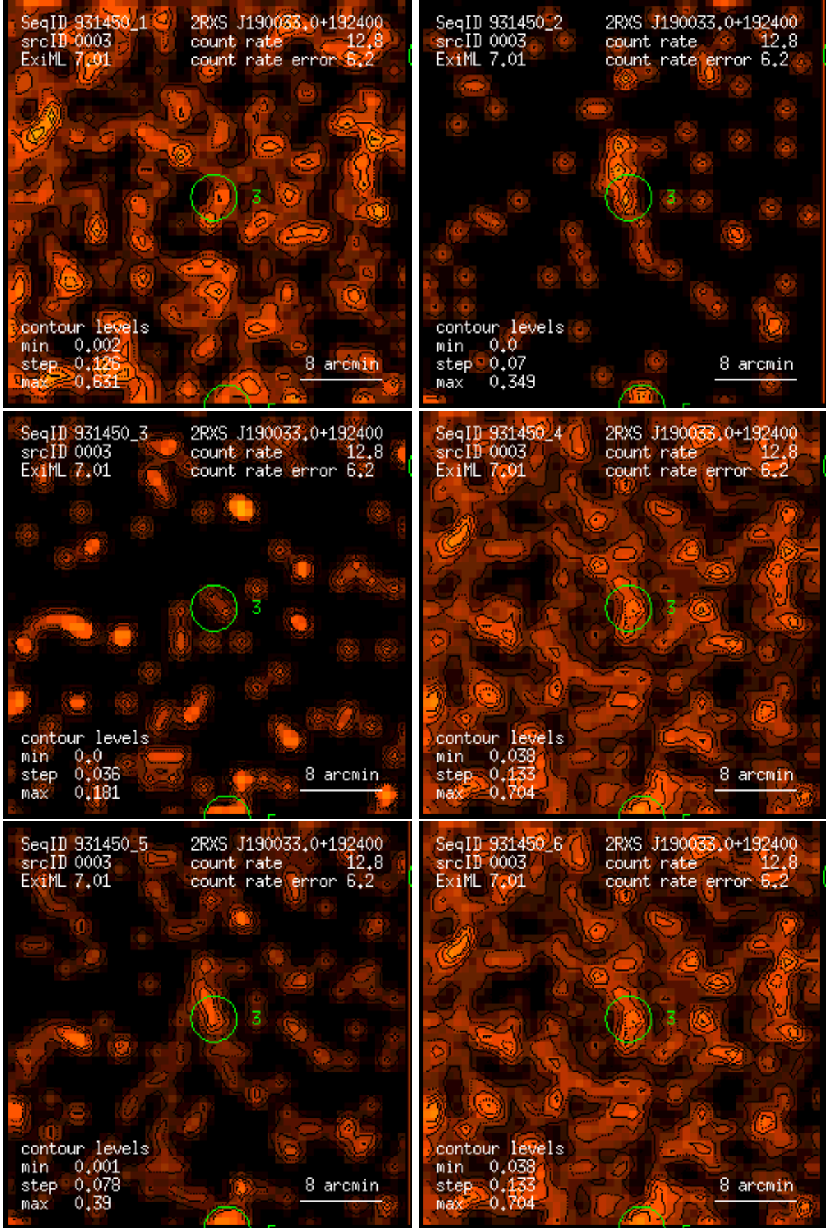
Figure 3: RASS 931450: detection 0003: band rate images, Gaussian filter: (1) PSPC channels 11 – 41, (2) 52 – 90, (3) 91 – 201, (4) 11 – 235, (5) 52 – 201, (6) 11 – 201. Broad band rates in counts/ks. Band rate contour levels in counts/ks/arcmin 2 .
