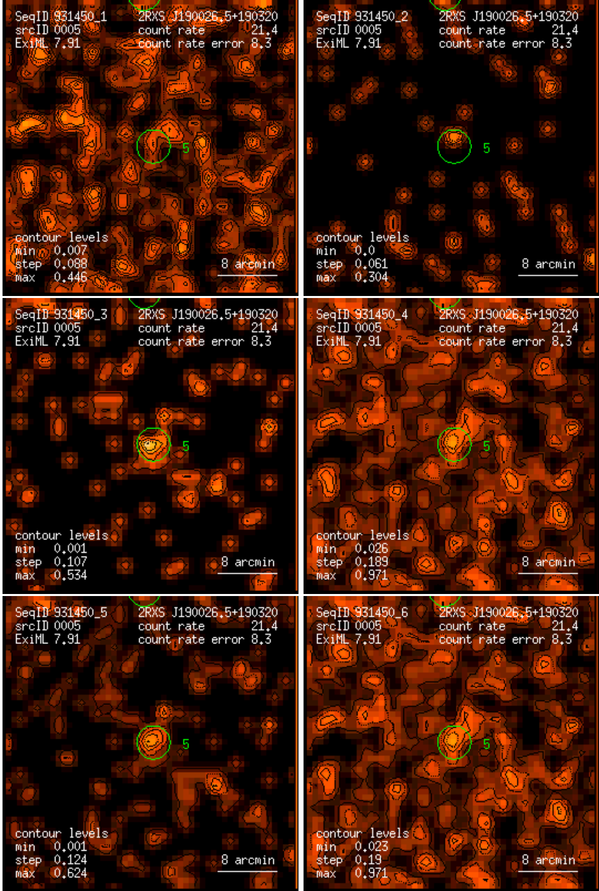
Figure 5: RASS 931450: detection 0005: band rate images, Gaussian filter: (1) PSPC channels 11 – 41, (2) 52 – 90, (3) 91 – 201, (4) 11 – 235, (5) 52 – 201, (6) 11 – 201. Broad band rates in counts/ks. Band rate contour levels in counts/ks/arcmin 2 .
