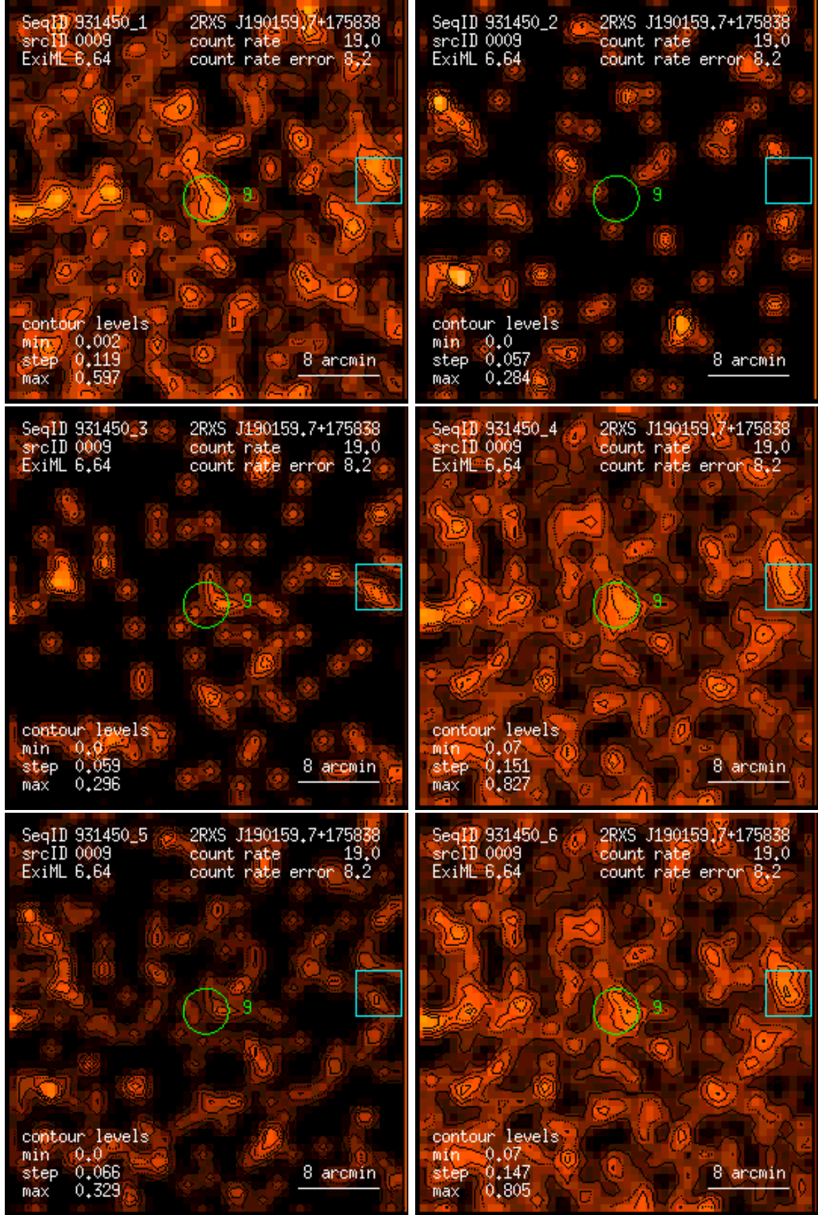
Figure 9: RASS 931450: detection 0009: band rate images, Gaussian filter: (1) PSPC channels 11 – 41, (2) 52 – 90, (3) 91 – 201, (4) 11 – 235, (5) 52 – 201, (6) 11 – 201. Broad band rates in counts/ks. Band rate contour levels in counts/ks/arcmin 2 .
