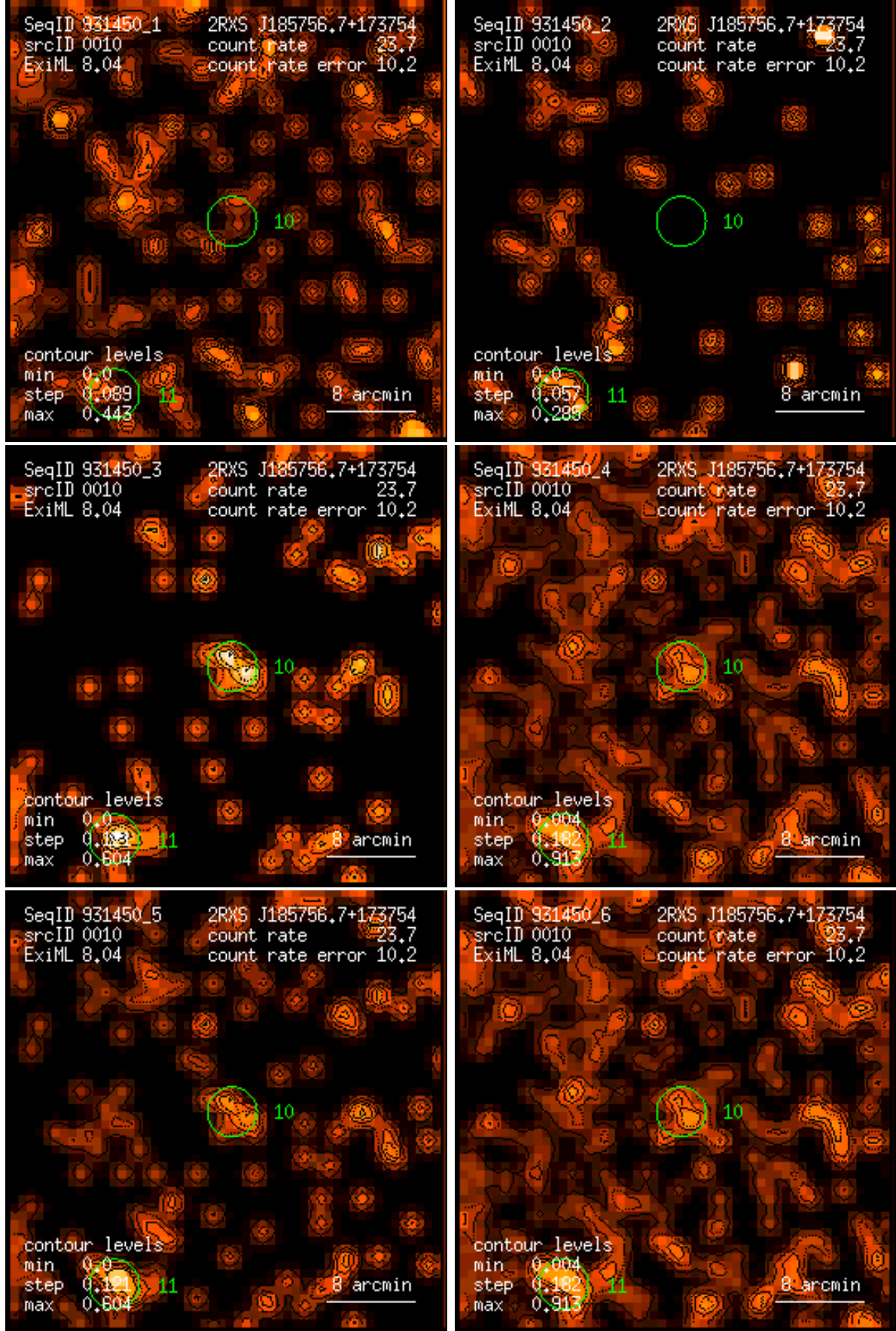
Figure 10: RASS 931450: detection 0010: band rate images, Gaussian filter: (1) PSPC channels 11 – 41, (2) 52 – 90, (3) 91 – 201, (4) 11 – 235, (5) 52 – 201, (6) 11 – 201. Broad band rates in counts/ks. Band rate contour levels in counts/ks/arcmin 2 .
