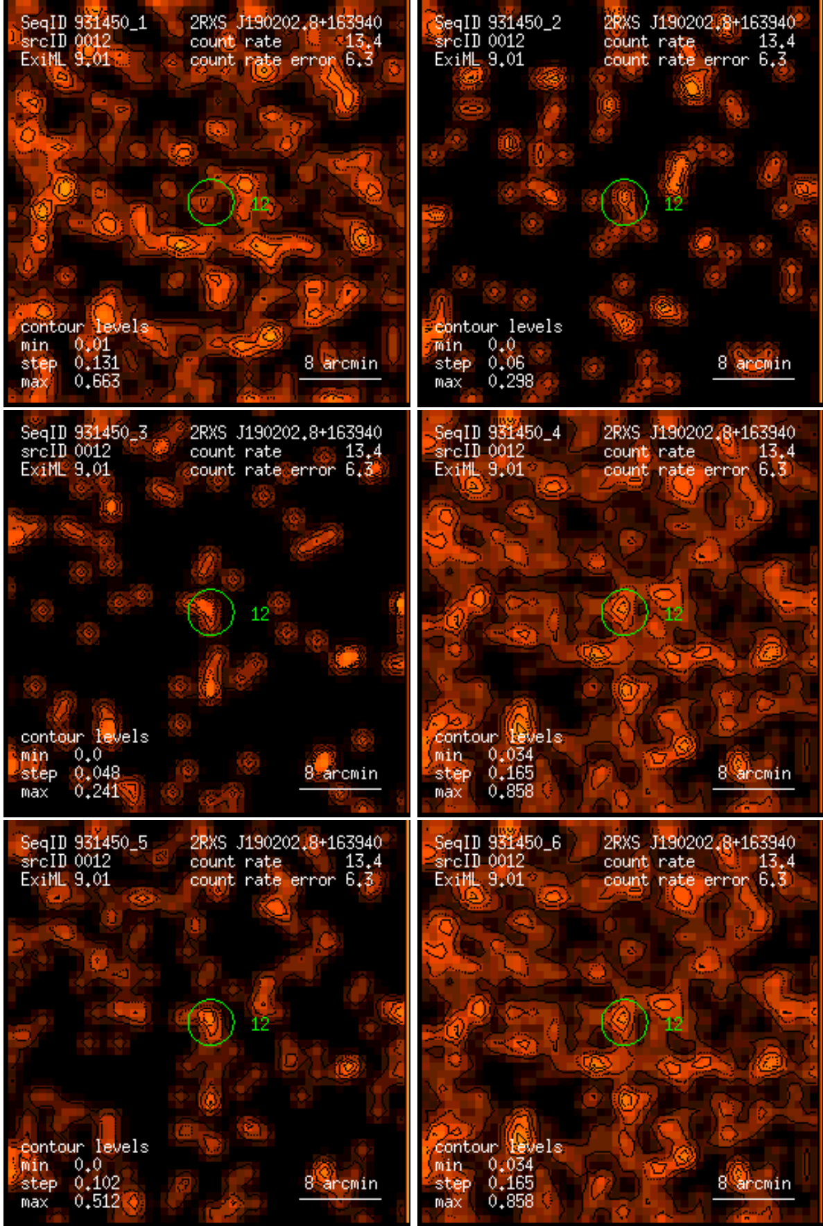
Figure 12: RASS 931450: detection 0012: band rate images, Gaussian filter: (1) PSPC channels 11 – 41, (2) 52 – 90, (3) 91 – 201, (4) 11 – 235, (5) 52 – 201, (6) 11 – 201. Broad band rates in counts/ks. Band rate contour levels in counts/ks/arcmin 2 .
