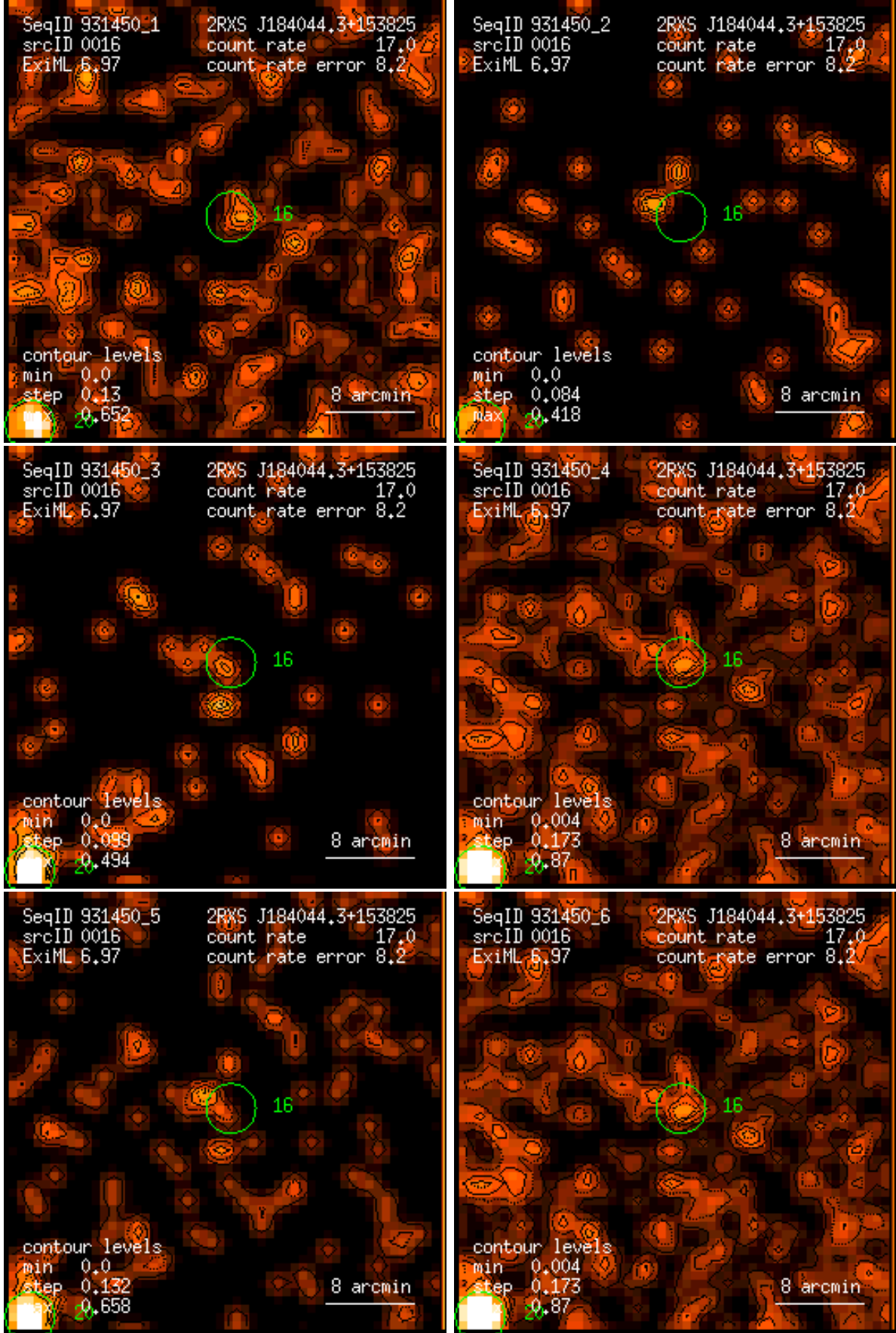
Figure 16: RASS 931450: detection 0016: band rate images, Gaussian filter: (1) PSPC channels 11 – 41, (2) 52 – 90, (3) 91 – 201, (4) 11 – 235, (5) 52 – 201, (6) 11 – 201. Broad band rates in counts/ks. Band rate contour levels in counts/ks/arcmin 2 .
