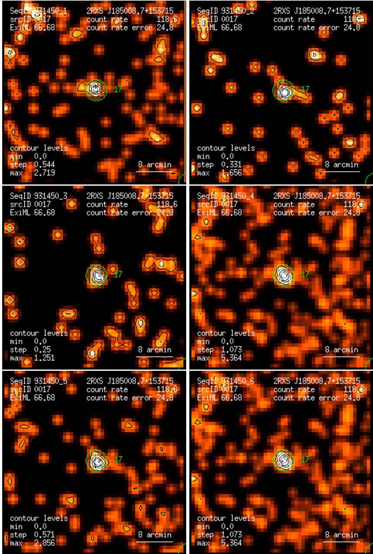
Figure 17: RASS 931450: detection 0017: band rate images, Gaussian filter: (1) PSPC channels 11 – 41, (2) 52 – 90, (3) 91 – 201, (4) 11 – 235, (5) 52 – 201, (6) 11 – 201. Broad band rates in counts/ks. Band rate contour levels in counts/ks/arcmin 2 .
