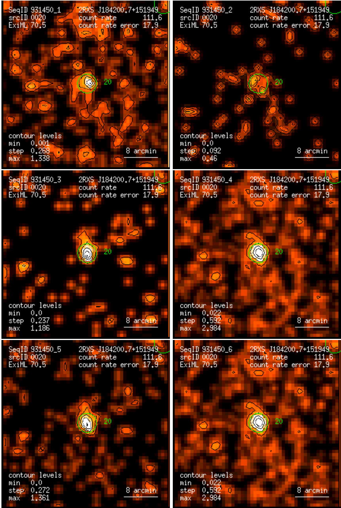
Figure 20: RASS 931450: detection 0020: band rate images, Gaussian filter: (1) PSPC channels 11 – 41, (2) 52 – 90, (3) 91 – 201, (4) 11 – 235, (5) 52 – 201, (6) 11 – 201. Broad band rates in counts/ks. Band rate contour levels in counts/ks/arcmin 2 .
