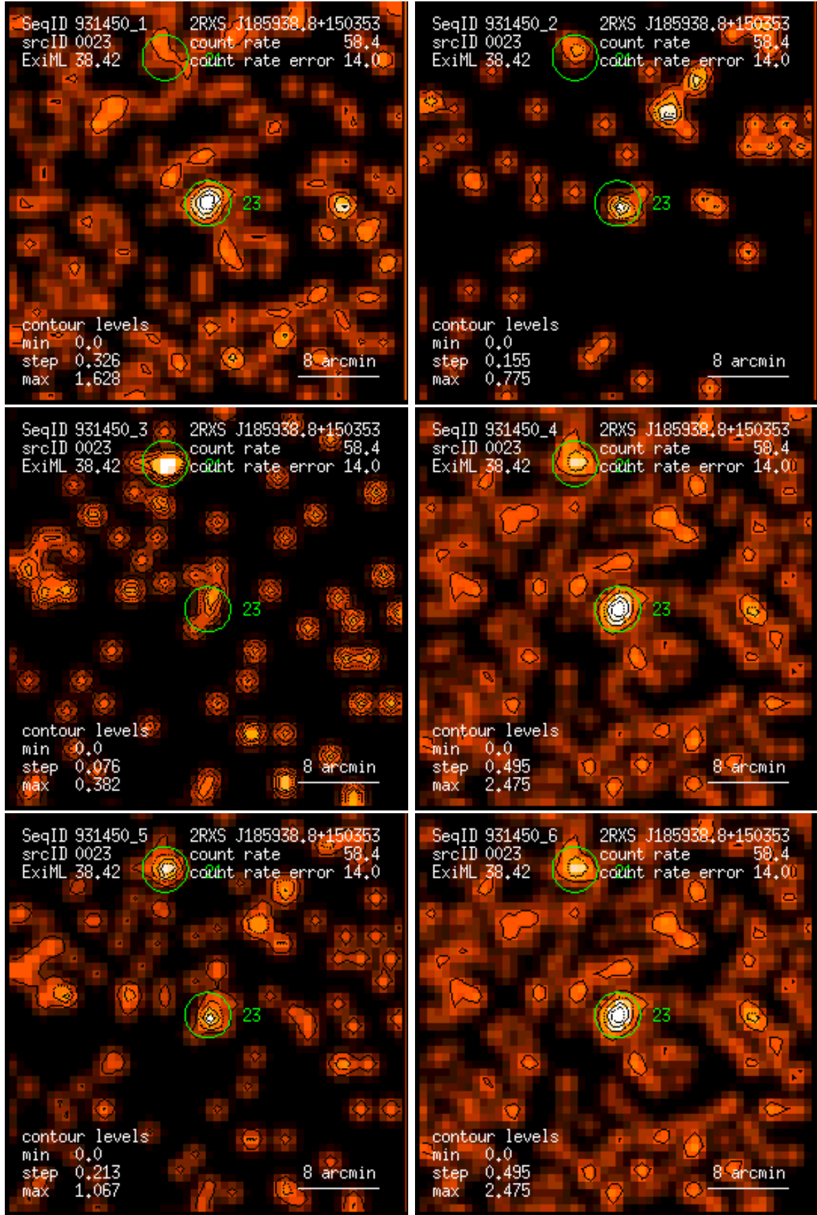
Figure 23: RASS 931450: detection 0023: band rate images, Gaussian filter: (1) PSPC channels 11 – 41, (2) 52 – 90, (3) 91 – 201, (4) 11 – 235, (5) 52 – 201, (6) 11 – 201. Broad band rates in counts/ks. Band rate contour levels in counts/ks/arcmin 2 .
