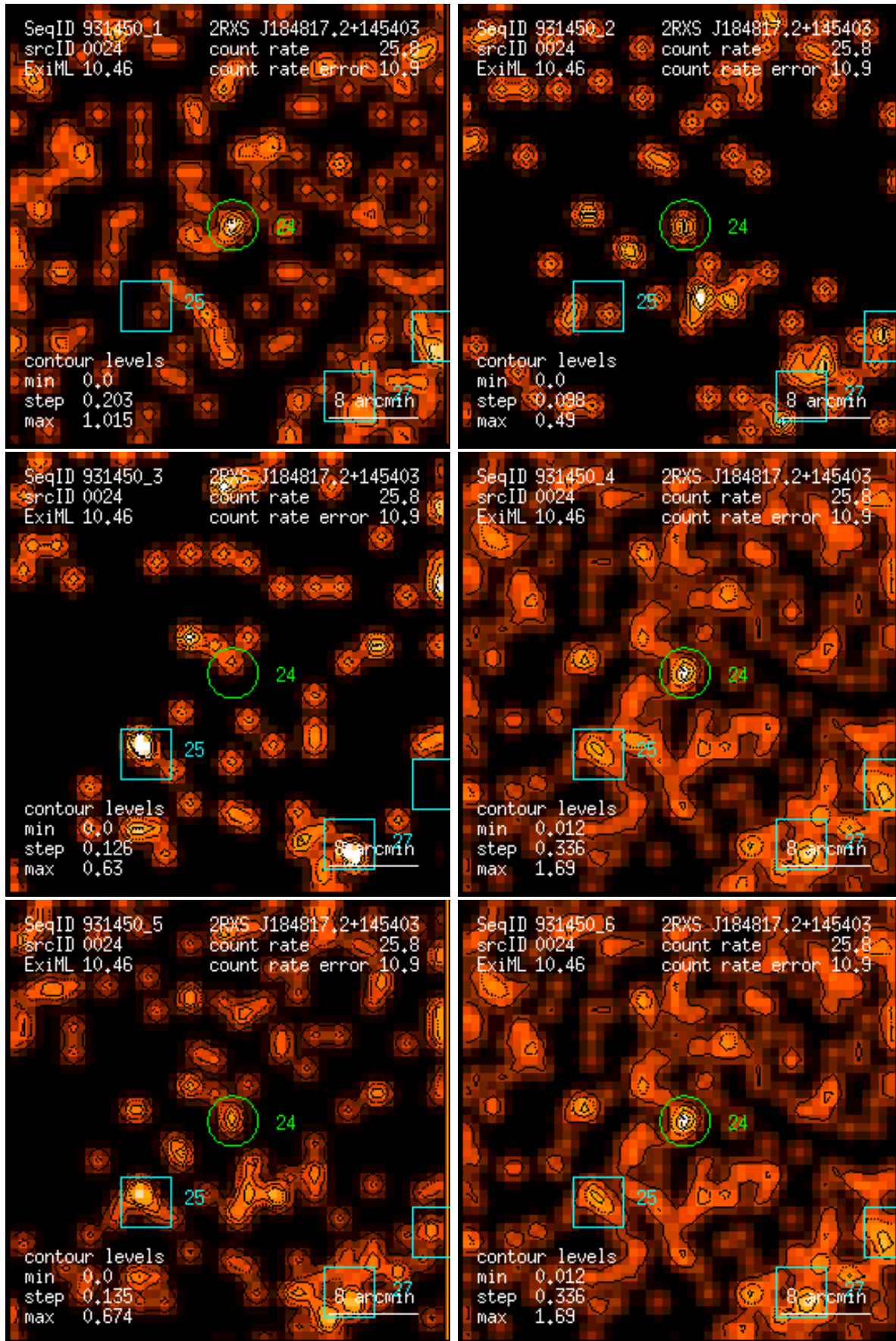
Figure 24: RASS 931450: detection 0024: band rate images, Gaussian filter: (1) PSPC channels 11 – 41, (2) 52 – 90, (3) 91 – 201, (4) 11 – 235, (5) 52 – 201, (6) 11 – 201. Broad band rates in counts/ks. Band rate contour levels in counts/ks/arcmin 2 .
