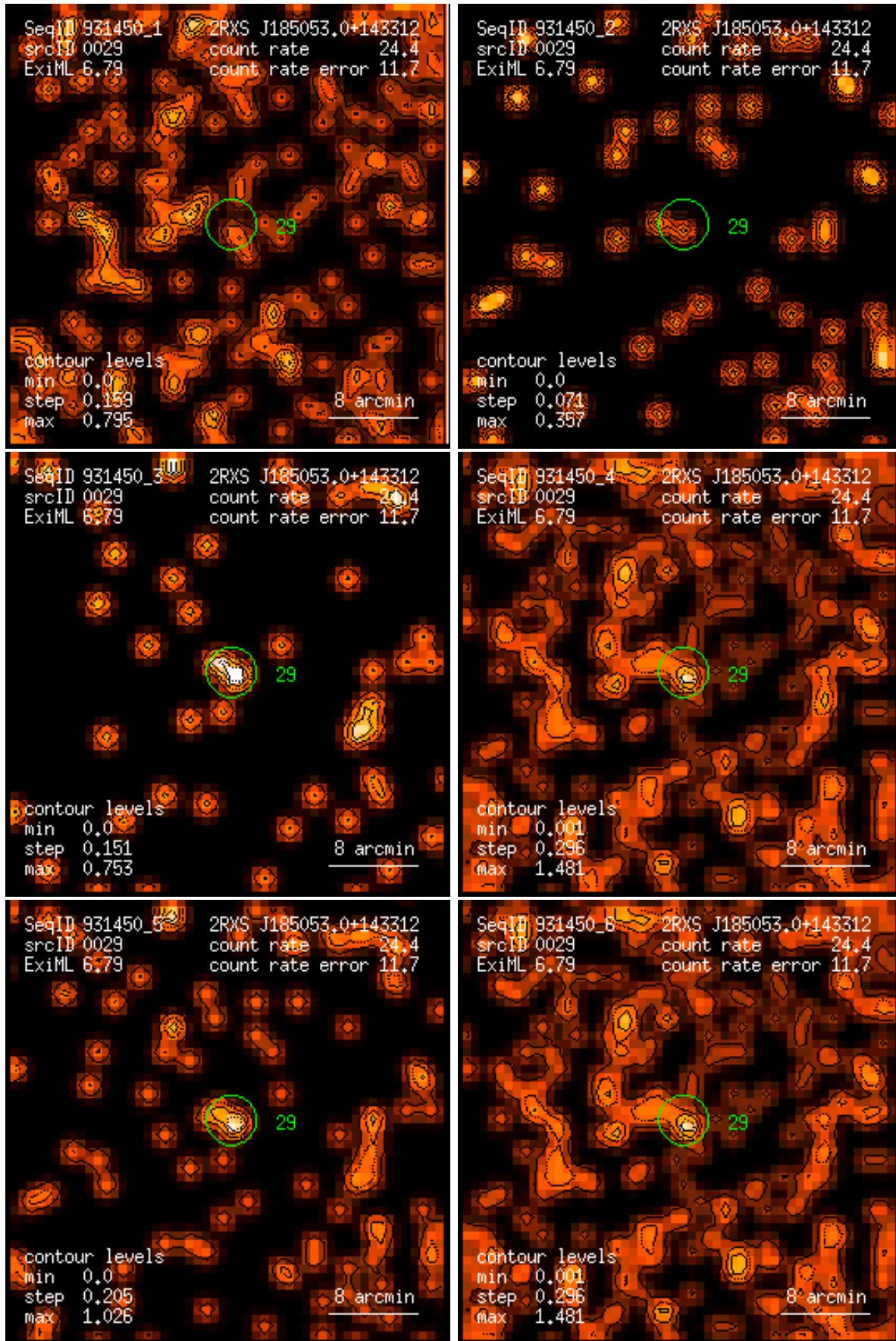
Figure 29: RASS 931450: detection 0029: band rate images, Gaussian filter: (1) PSPC channels 11 – 41, (2) 52 – 90, (3) 91 – 201, (4) 11 – 235, (5) 52 – 201, (6) 11 – 201. Broad band rates in counts/ks. Band rate contour levels in counts/ks/arcmin 2 .
