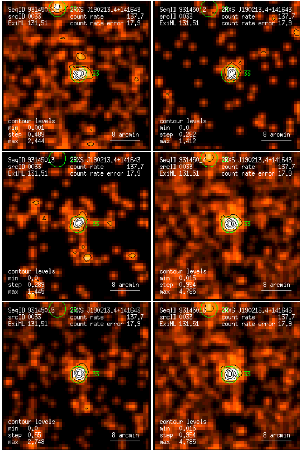
Figure 33: RASS 931450: detection 0033: band rate images, Gaussian filter: (1) PSPC channels 11 – 41, (2) 52 – 90, (3) 91 – 201, (4) 11 – 235, (5) 52 – 201, (6) 11 – 201. Broad band rates in counts/ks. Band rate contour levels in counts/ks/arcmin 2 .
