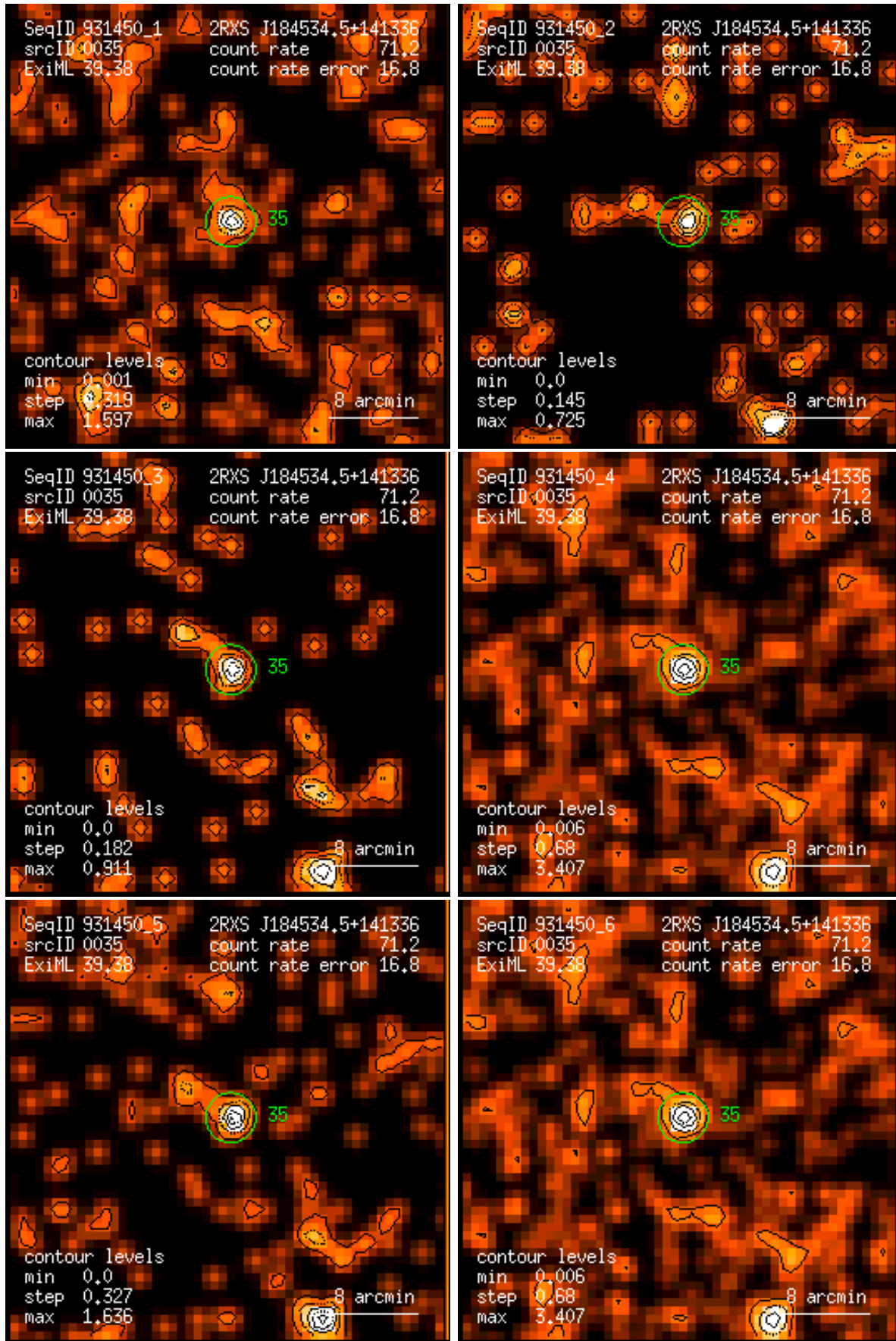
Figure 35: RASS 931450: detection 0035: band rate images, Gaussian filter: (1) PSPC channels 11 – 41, (2) 52 – 90, (3) 91 – 201, (4) 11 – 235, (5) 52 – 201, (6) 11 – 201. Broad band rates in counts/ks. Band rate contour levels in counts/ks/arcmin 2 .
