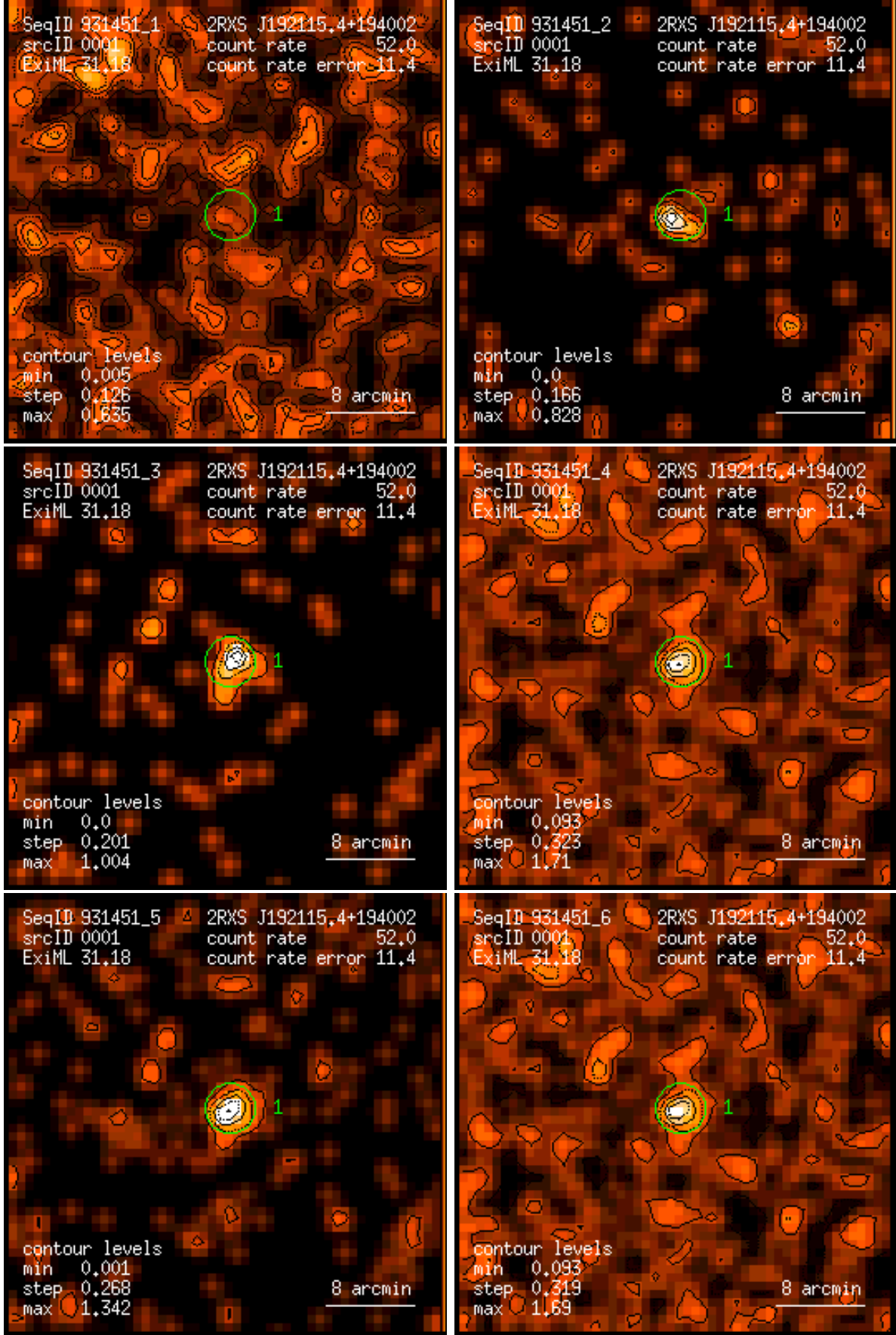
Figure 1: RASS 931451: detection 0001: band rate images, Gaussian filter: (1) PSPC channels 11 – 41, (2) 52 – 90, (3) 91 – 201, (4) 11 – 235, (5) 52 – 201, (6) 11 – 201. Broad band rates in counts/ks. Band rate contour levels in counts/ks/arcmin 2 .
