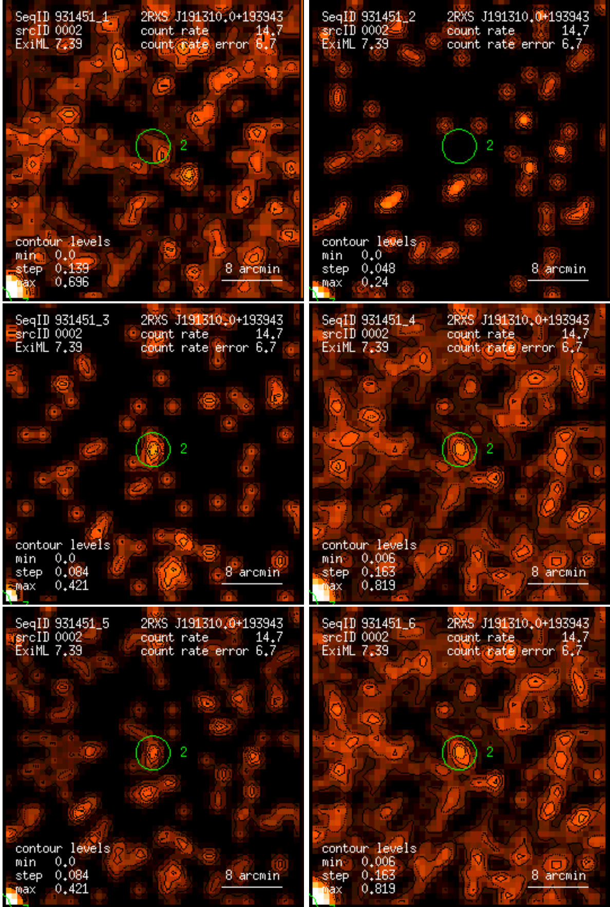
Figure 2: RASS 931451: detection 0002: band rate images, Gaussian filter: (1) PSPC channels 11 – 41, (2) 52 – 90, (3) 91 – 201, (4) 11 – 235, (5) 52 – 201, (6) 11 – 201. Broad band rates in counts/ks. Band rate contour levels in counts/ks/arcmin 2 .
