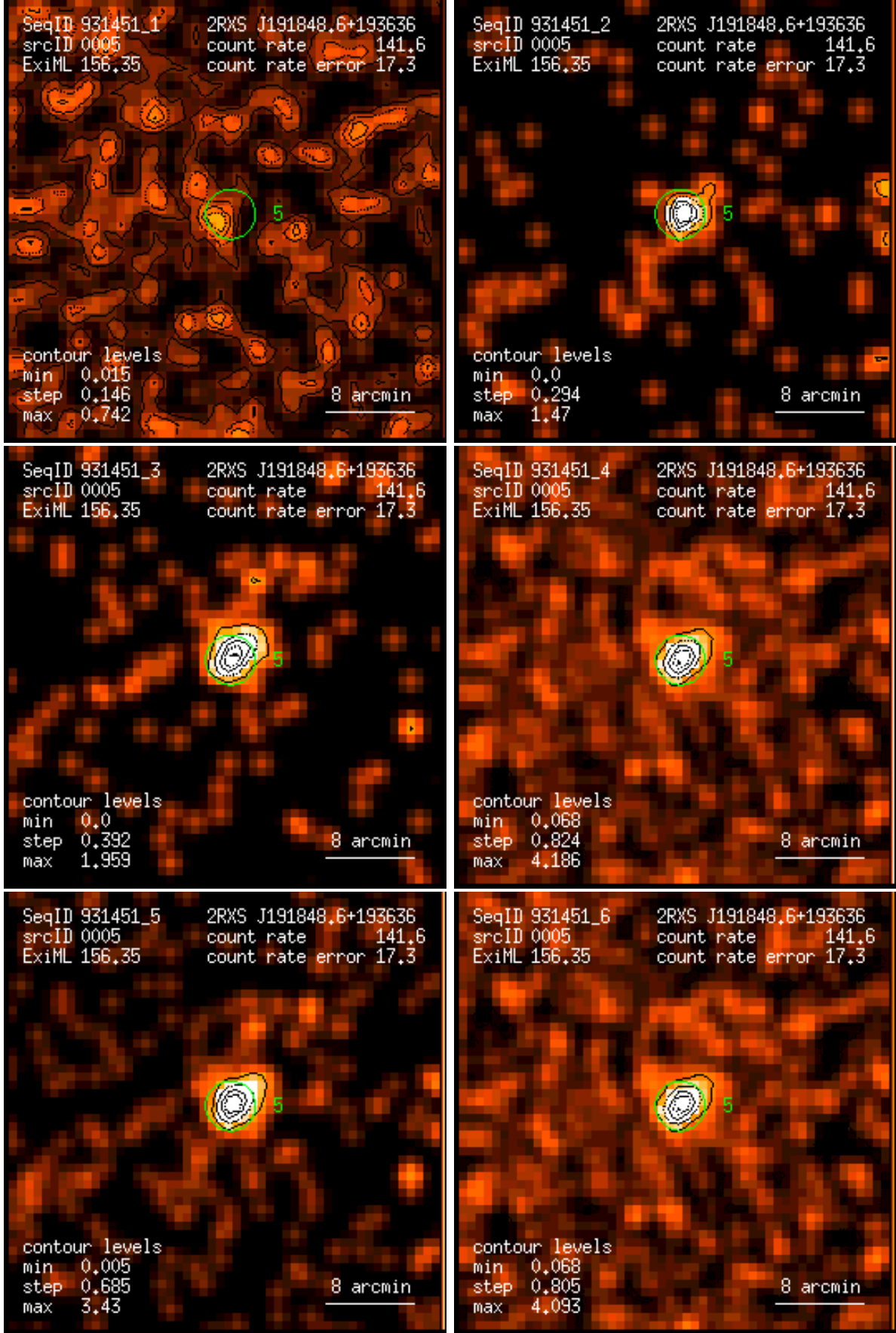
Figure 5: RASS 931451: detection 0005: band rate images, Gaussian filter: (1) PSPC channels 11 – 41, (2) 52 – 90, (3) 91 – 201, (4) 11 – 235, (5) 52 – 201, (6) 11 – 201. Broad band rates in counts/ks. Band rate contour levels in counts/ks/arcmin 2 .
