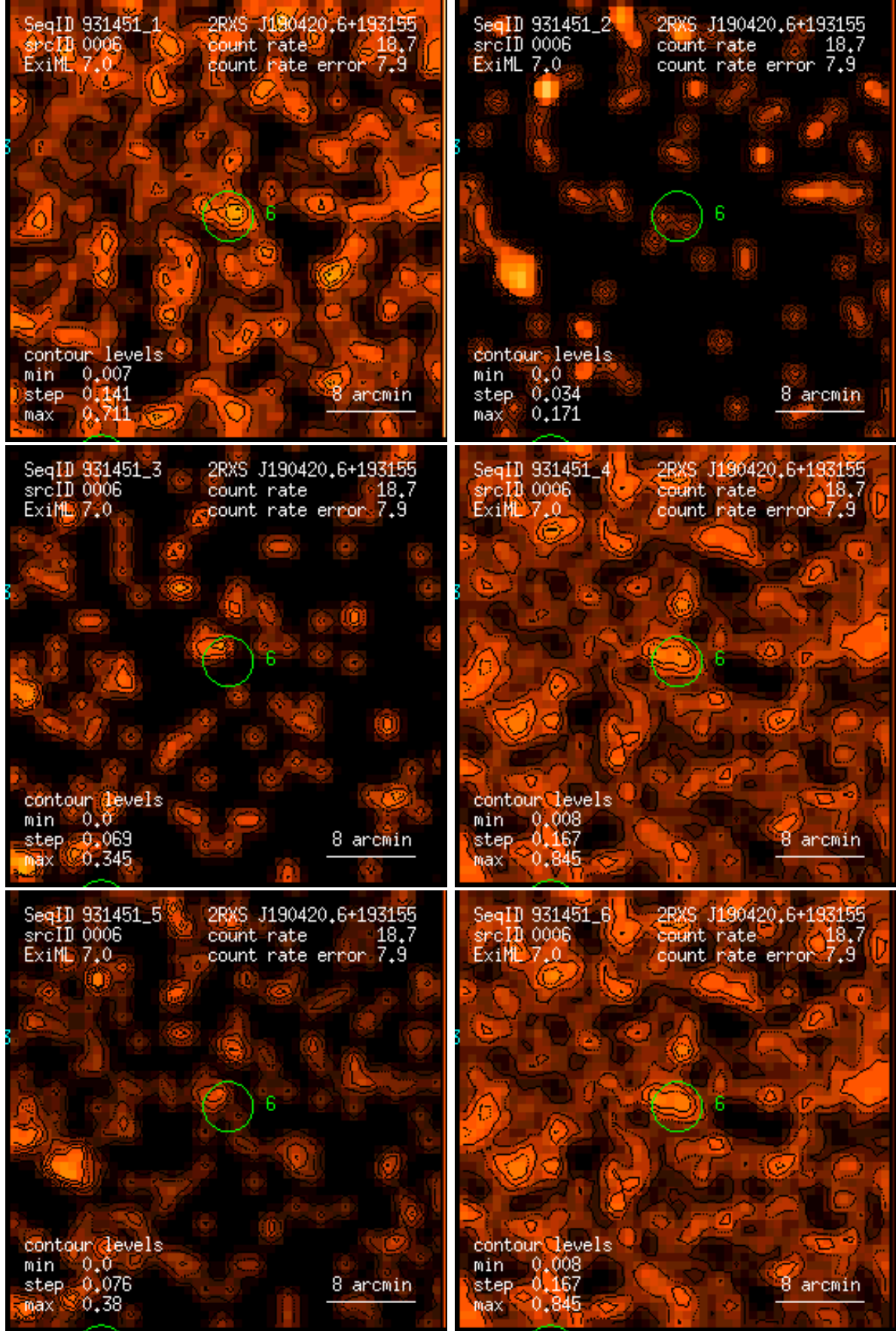
Figure 6: RASS 931451: detection 0006: band rate images, Gaussian filter: (1) PSPC channels 11 – 41, (2) 52 – 90, (3) 91 – 201, (4) 11 – 235, (5) 52 – 201, (6) 11 – 201. Broad band rates in counts/ks. Band rate contour levels in counts/ks/arcmin 2 .
