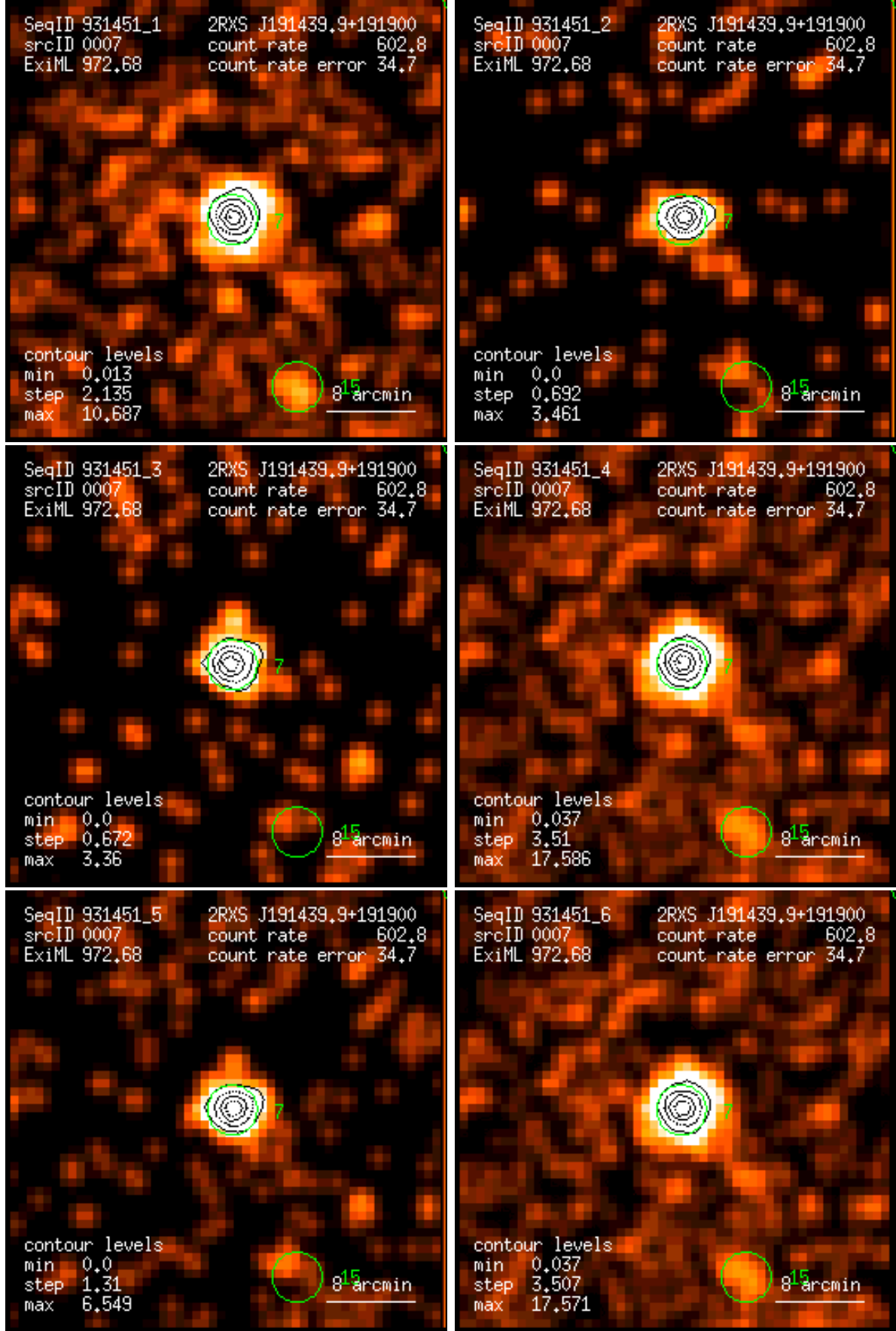
Figure 7: RASS 931451: detection 0007: band rate images, Gaussian filter: (1) PSPC channels 11 – 41, (2) 52 – 90, (3) 91 – 201, (4) 11 – 235, (5) 52 – 201, (6) 11 – 201. Broad band rates in counts/ks. Band rate contour levels in counts/ks/arcmin 2 .
