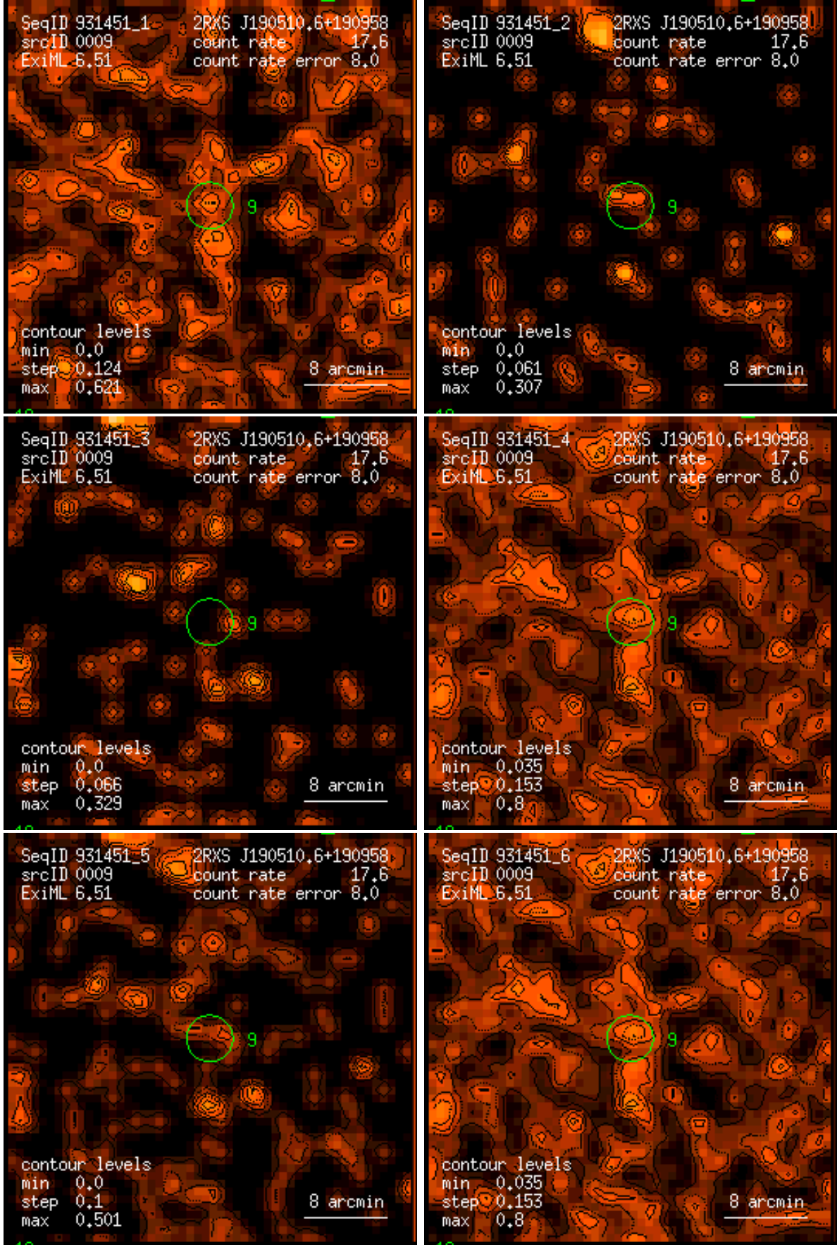
Figure 9: RASS 931451: detection 0009: band rate images, Gaussian filter: (1) PSPC channels 11 – 41, (2) 52 – 90, (3) 91 – 201, (4) 11 – 235, (5) 52 – 201, (6) 11 – 201. Broad band rates in counts/ks. Band rate contour levels in counts/ks/arcmin 2 .
